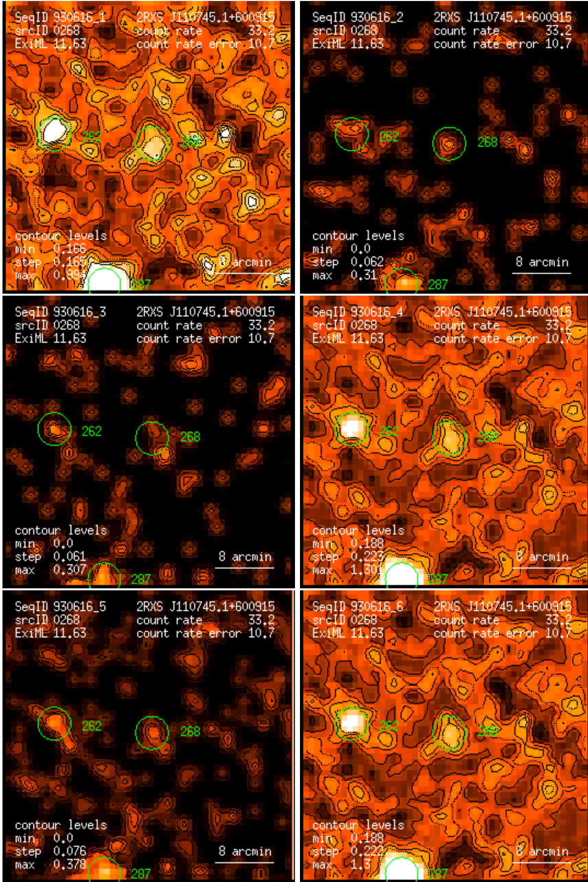
Figure 268: RASS 930616: detection 0268: band rate images, Gaussian filter: (1) PSPC channels 11 – 41, (2) 52 – 90, (3) 91 – 201, (4) 11 – 235, (5) 52 – 201, (6) 11 – 201. Broad band rates in counts/ks. Band rate contour levels in counts/ks/arcmin 2 .
