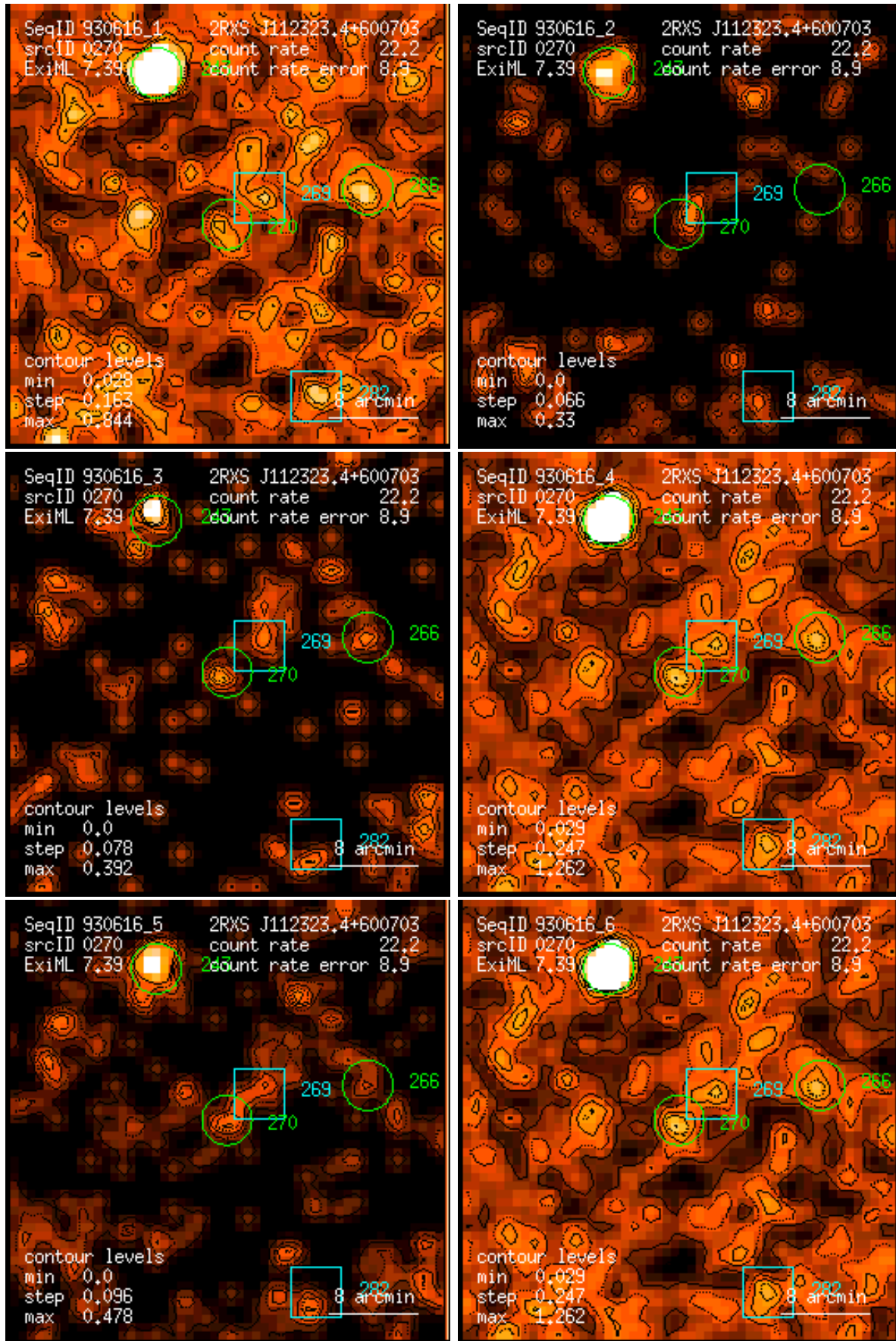
Figure 270: RASS 930616: detection 0270: band rate images, Gaussian filter: (1) PSPC channels 11 – 41, (2) 52 – 90, (3) 91 – 201, (4) 11 – 235, (5) 52 – 201, (6) 11 – 201. Broad band rates in counts/ks. Band rate contour levels in counts/ks/arcmin 2 .
