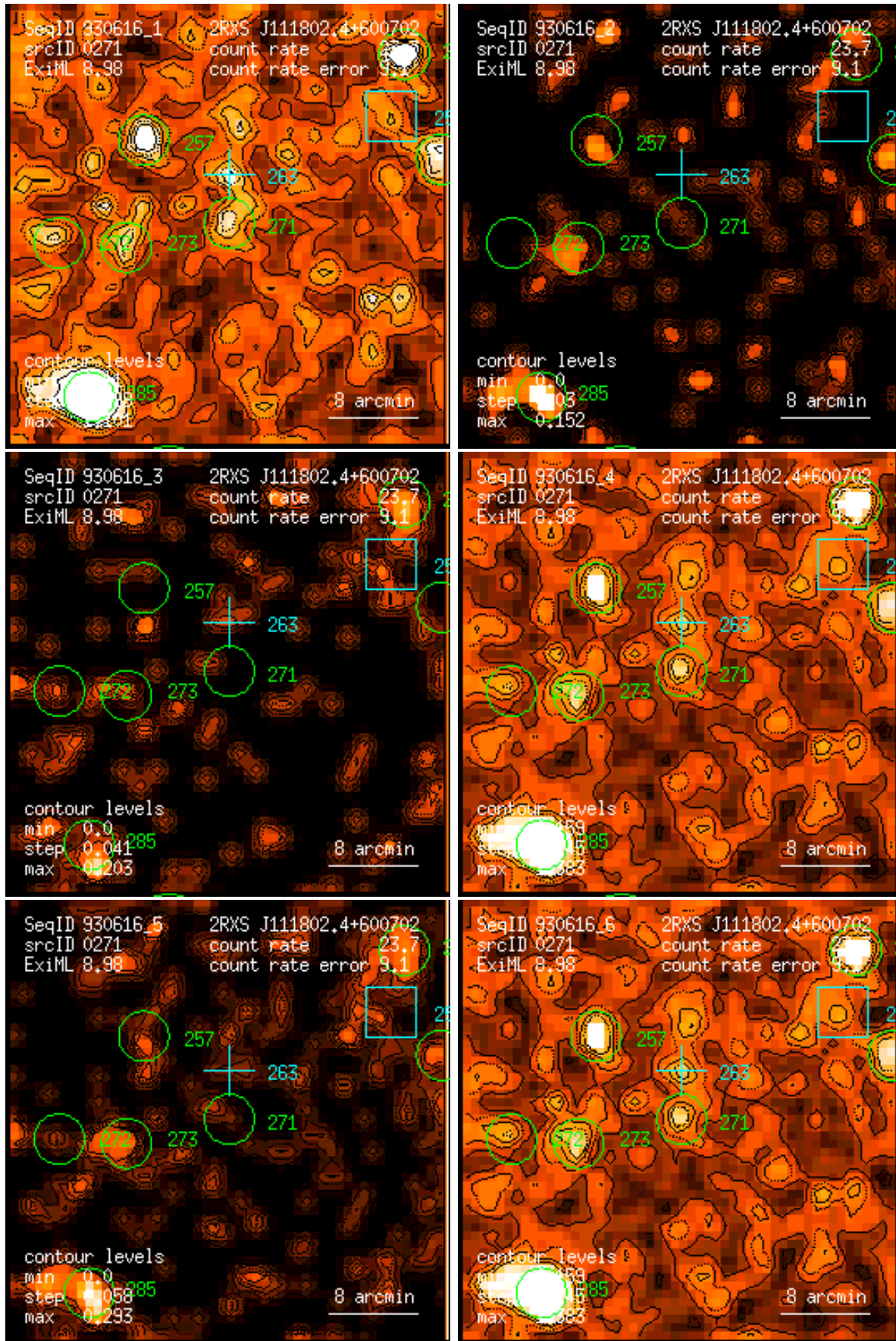
Figure 271: RASS 930616: detection 0271: band rate images, Gaussian filter: (1) PSPC channels 11 – 41, (2) 52 – 90, (3) 91 – 201, (4) 11 – 235, (5) 52 – 201, (6) 11 – 201. Broad band rates in counts/ks. Band rate contour levels in counts/ks/arcmin 2 .
