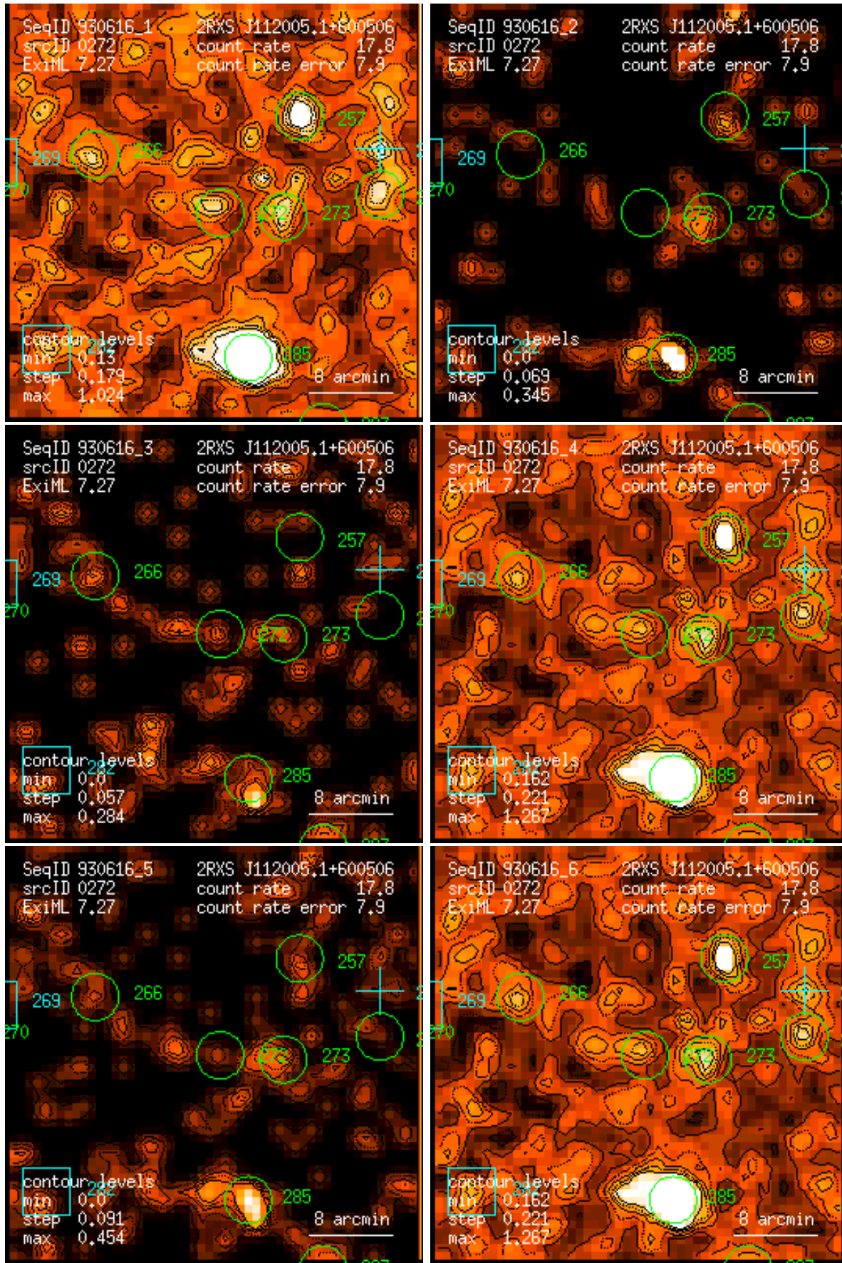
Figure 272: RASS 930616: detection 0272: band rate images, Gaussian filter: (1) PSPC channels 11 – 41, (2) 52 – 90, (3) 91 – 201, (4) 11 – 235, (5) 52 – 201, (6) 11 – 201. Broad band rates in counts/ks. Band rate contour levels in counts/ks/arcmin 2 .
