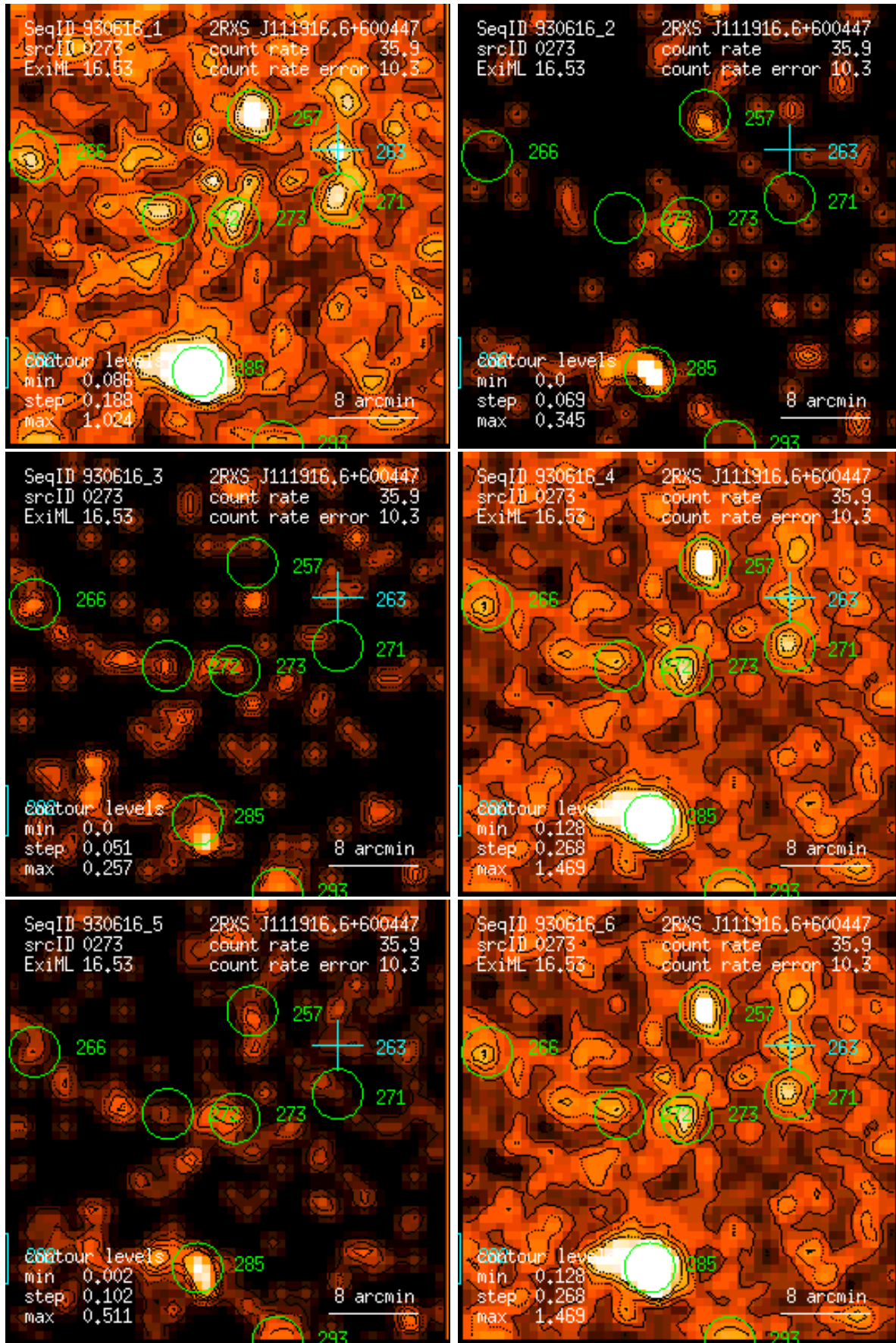
Figure 273: RASS 930616: detection 0273: band rate images, Gaussian filter: (1) PSPC channels 11 – 41, (2) 52 – 90, (3) 91 – 201, (4) 11 – 235, (5) 52 – 201, (6) 11 – 201. Broad band rates in counts/ks. Band rate contour levels in counts/ks/arcmin 2 .
