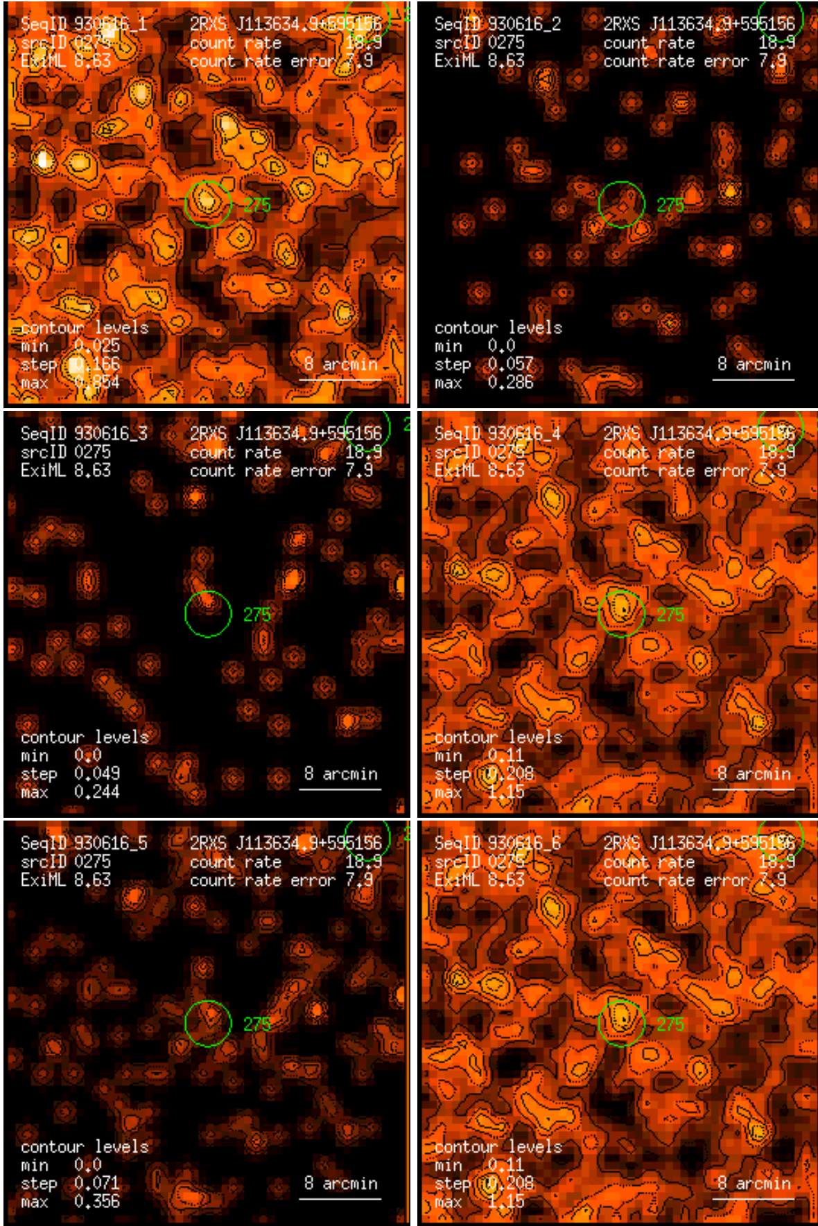
Figure 275: RASS 930616: detection 0275: band rate images, Gaussian filter: (1) PSPC channels 11 – 41, (2) 52 – 90, (3) 91 – 201, (4) 11 – 235, (5) 52 – 201, (6) 11 – 201. Broad band rates in counts/ks. Band rate contour levels in counts/ks/arcmin 2 .
