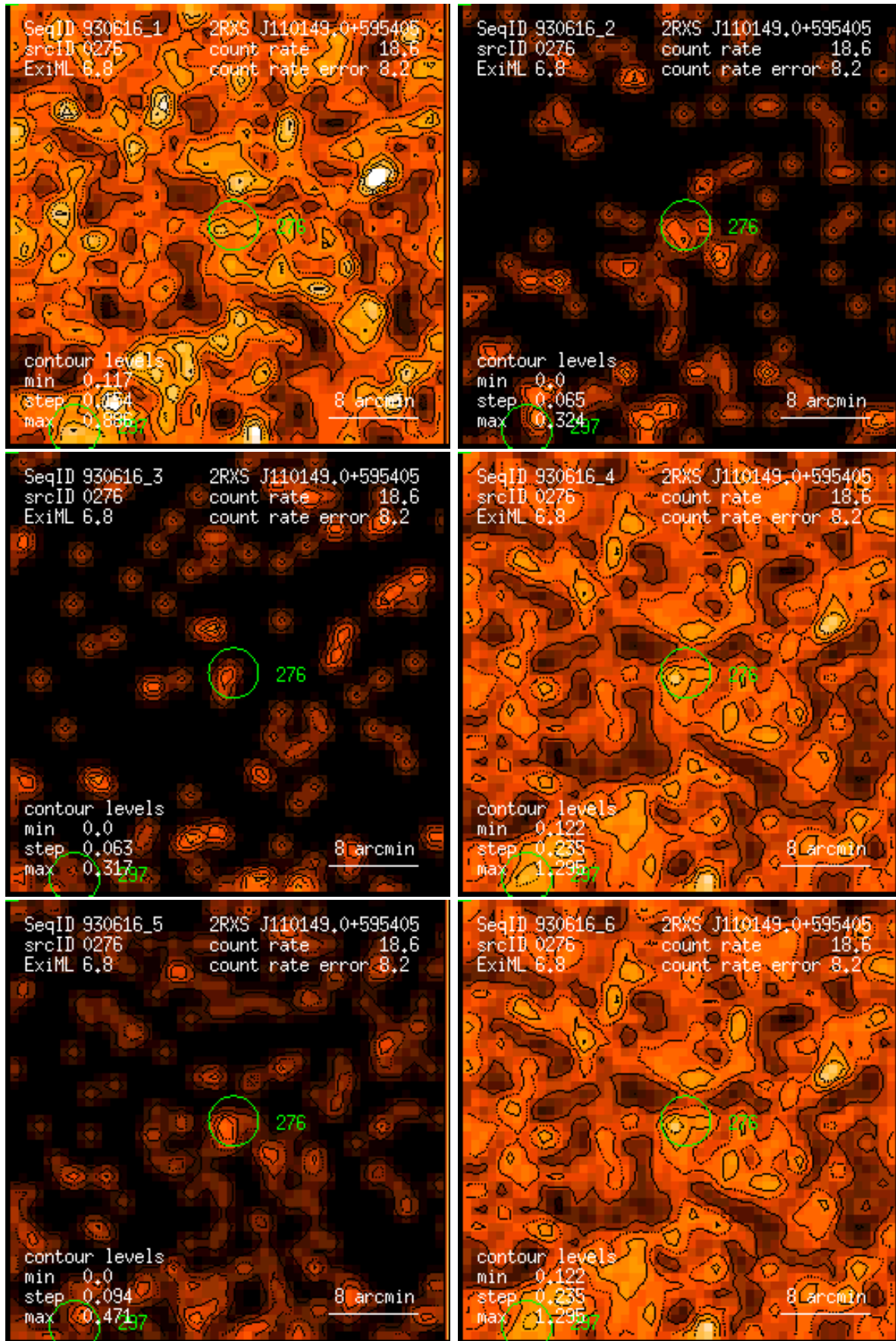
Figure 276: RASS 930616: detection 0276: band rate images, Gaussian filter: (1) PSPC channels 11 – 41, (2) 52 – 90, (3) 91 – 201, (4) 11 – 235, (5) 52 – 201, (6) 11 – 201. Broad band rates in counts/ks. Band rate contour levels in counts/ks/arcmin 2 .
