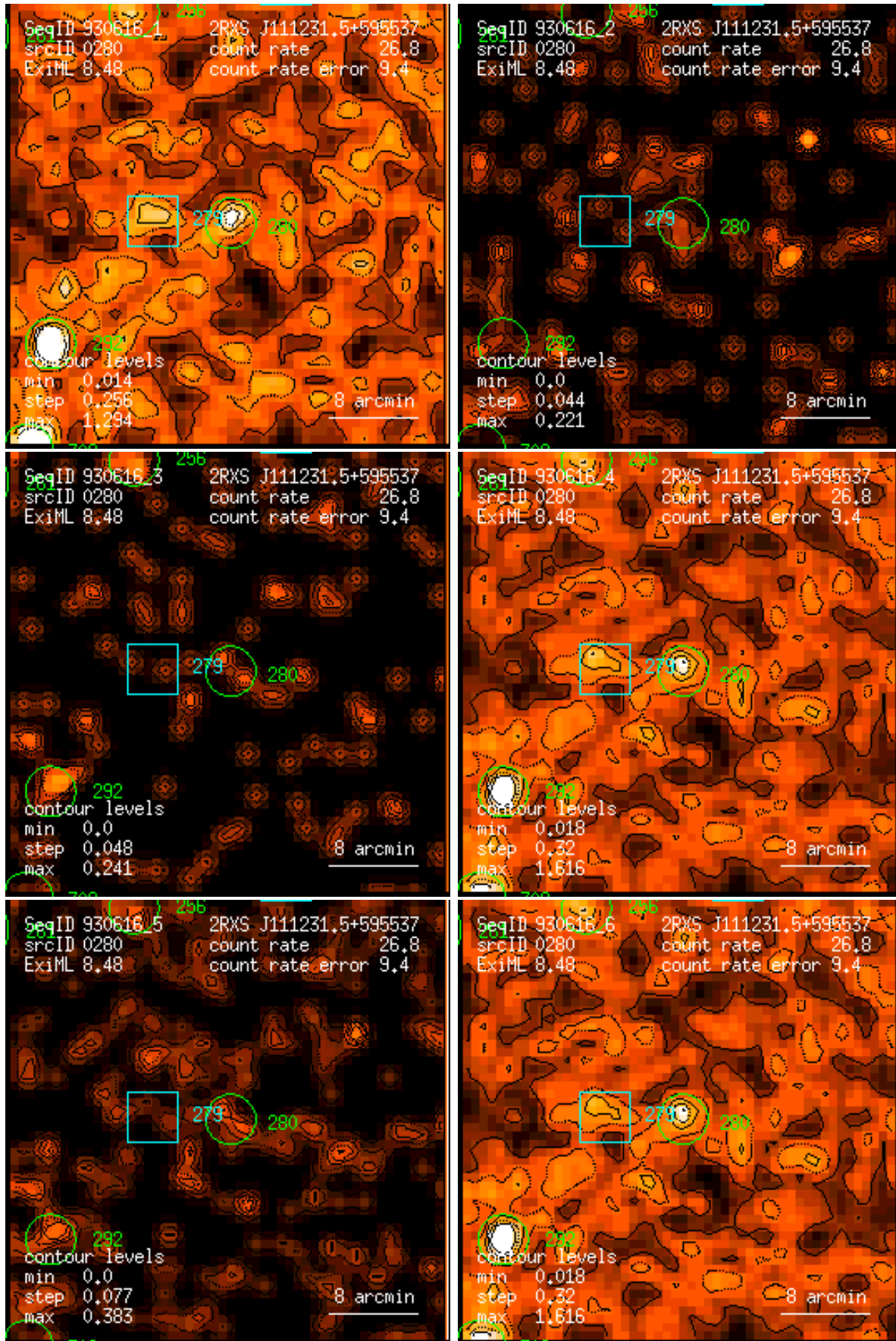
Figure 280: RASS 930616: detection 0280: band rate images, Gaussian filter: (1) PSPC channels 11 – 41, (2) 52 – 90, (3) 91 – 201, (4) 11 – 235, (5) 52 – 201, (6) 11 – 201. Broad band rates in counts/ks. Band rate contour levels in counts/ks/arcmin 2 .
