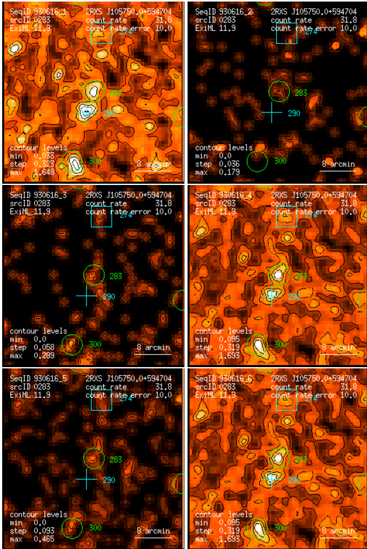
Figure 283: RASS 930616: detection 0283: band rate images, Gaussian filter: (1) PSPC channels 11 – 41, (2) 52 – 90, (3) 91 – 201, (4) 11 – 235, (5) 52 – 201, (6) 11 – 201. Broad band rates in counts/ks. Band rate contour levels in counts/ks/arcmin 2 .
