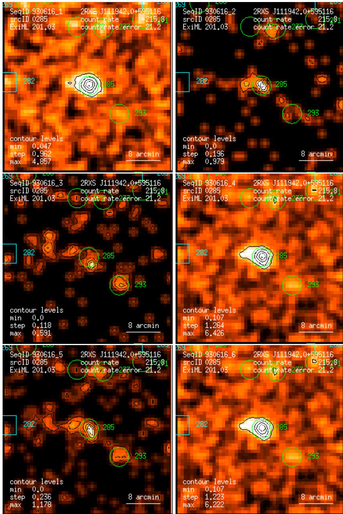
Figure 285: RASS 930616: detection 0285: band rate images, Gaussian filter: (1) PSPC channels 11 – 41, (2) 52 – 90, (3) 91 – 201, (4) 11 – 235, (5) 52 – 201, (6) 11 – 201. Broad band rates in counts/ks. Band rate contour levels in counts/ks/arcmin 2 .
