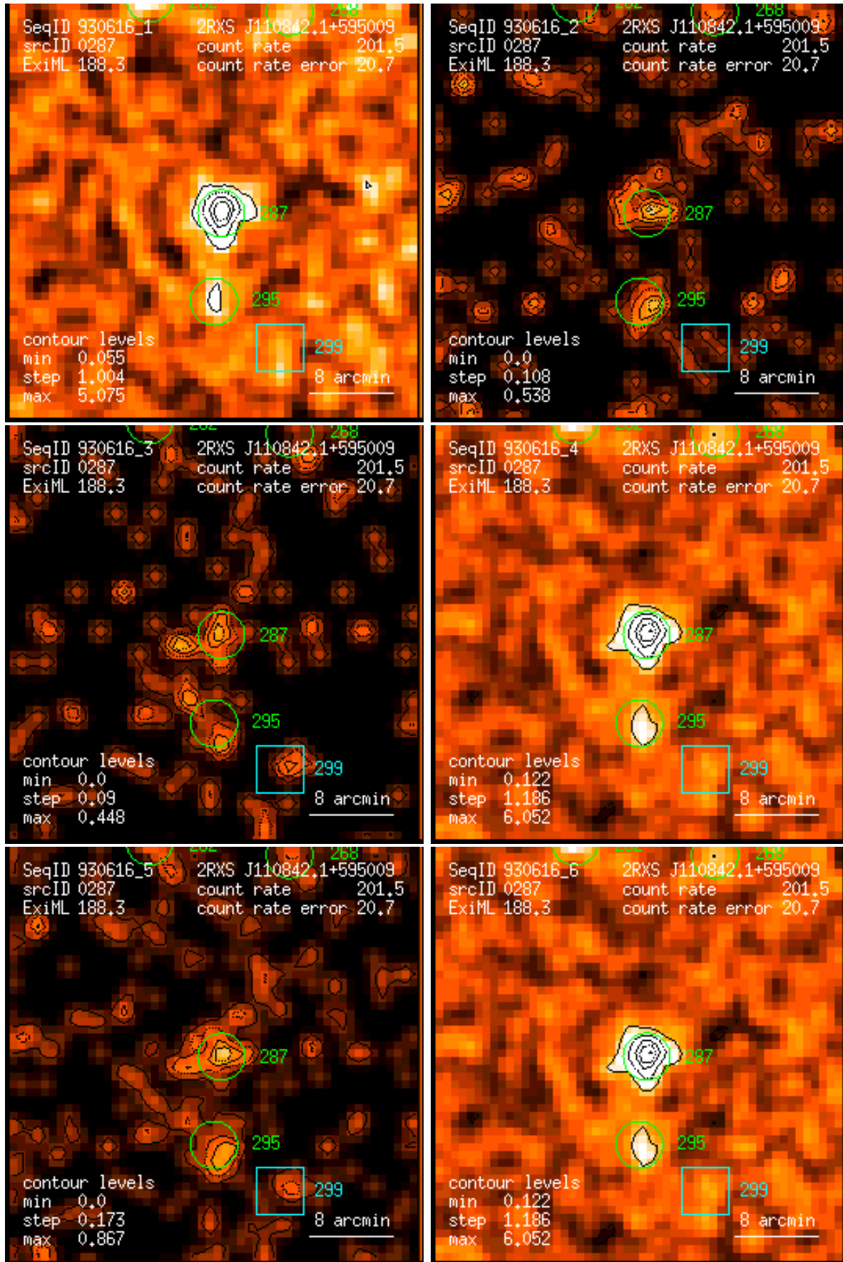
Figure 287: RASS 930616: detection 0287: band rate images, Gaussian filter: (1) PSPC channels 11 – 41, (2) 52 – 90, (3) 91 – 201, (4) 11 – 235, (5) 52 – 201, (6) 11 – 201. Broad band rates in counts/ks. Band rate contour levels in counts/ks/arcmin 2 .
