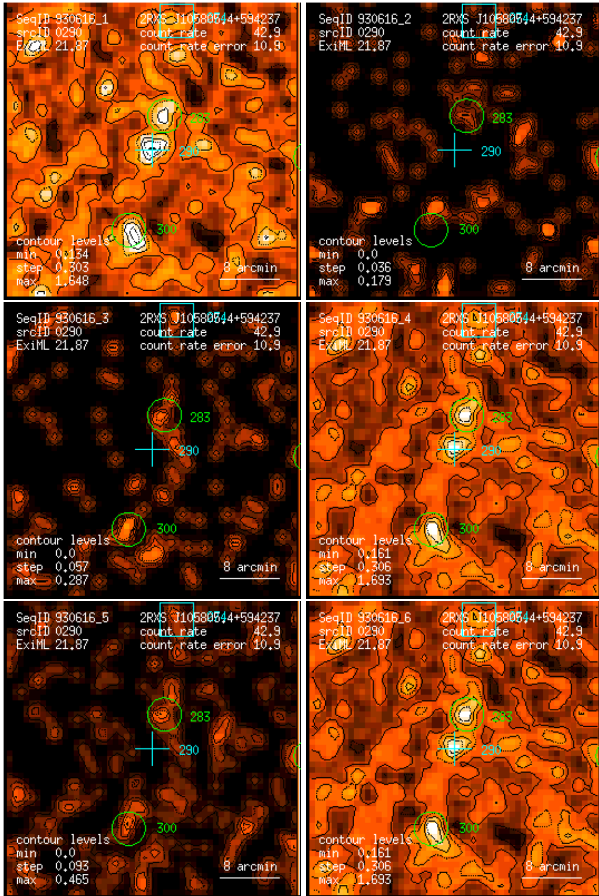
Figure 290: RASS 930616: detection 0290: band rate images, Gaussian filter: (1) PSPC channels 11 – 41, (2) 52 – 90, (3) 91 – 201, (4) 11 – 235, (5) 52 – 201, (6) 11 – 201. Broad band rates in counts/ks. Band rate contour levels in counts/ks/arcmin 2 .
