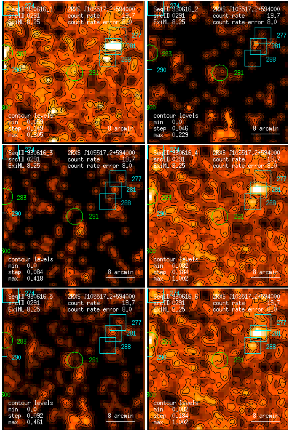
Figure 291: RASS 930616: detection 0291: band rate images, Gaussian filter: (1) PSPC channels 11 – 41, (2) 52 – 90, (3) 91 – 201, (4) 11 – 235, (5) 52 – 201, (6) 11 – 201. Broad band rates in counts/ks. Band rate contour levels in counts/ks/arcmin 2 .
