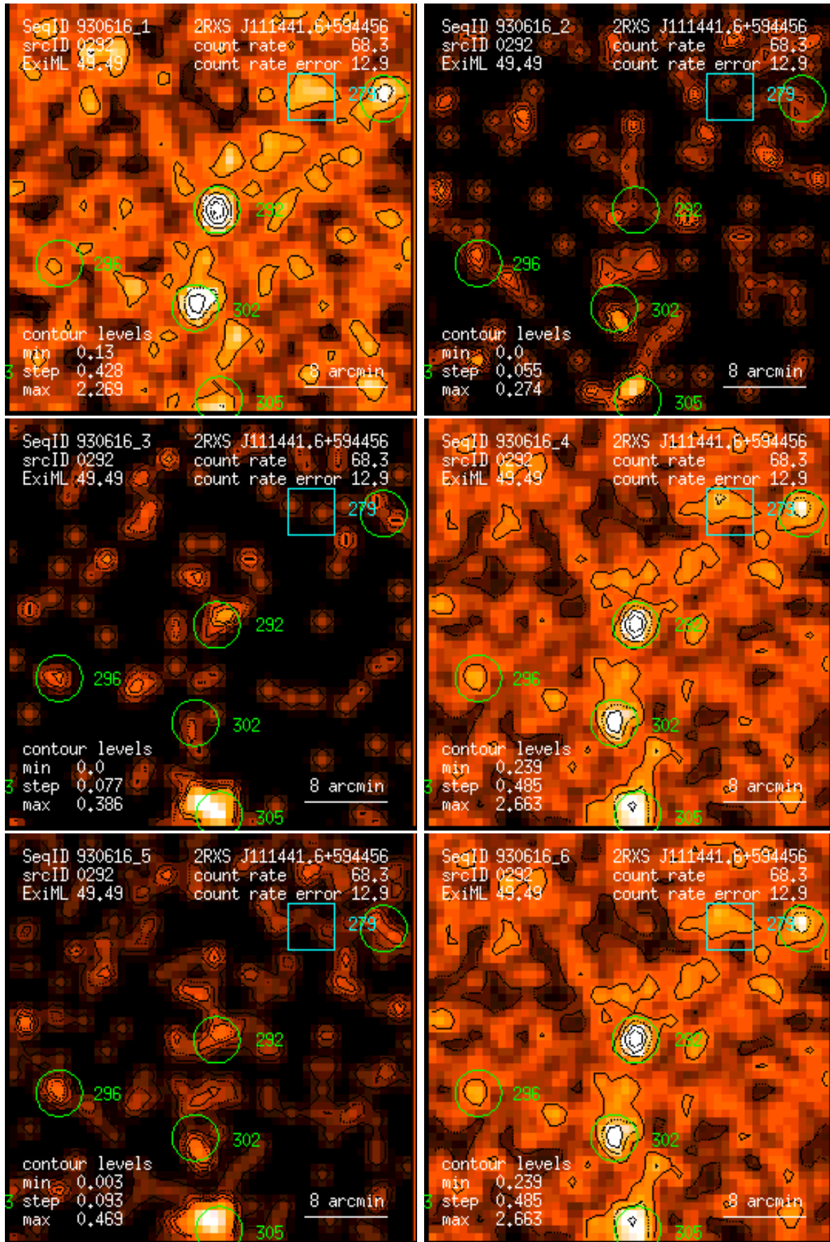
Figure 292: RASS 930616: detection 0292: band rate images, Gaussian filter: (1) PSPC channels 11 – 41, (2) 52 – 90, (3) 91 – 201, (4) 11 – 235, (5) 52 – 201, (6) 11 – 201. Broad band rates in counts/ks. Band rate contour levels in counts/ks/arcmin 2 .
