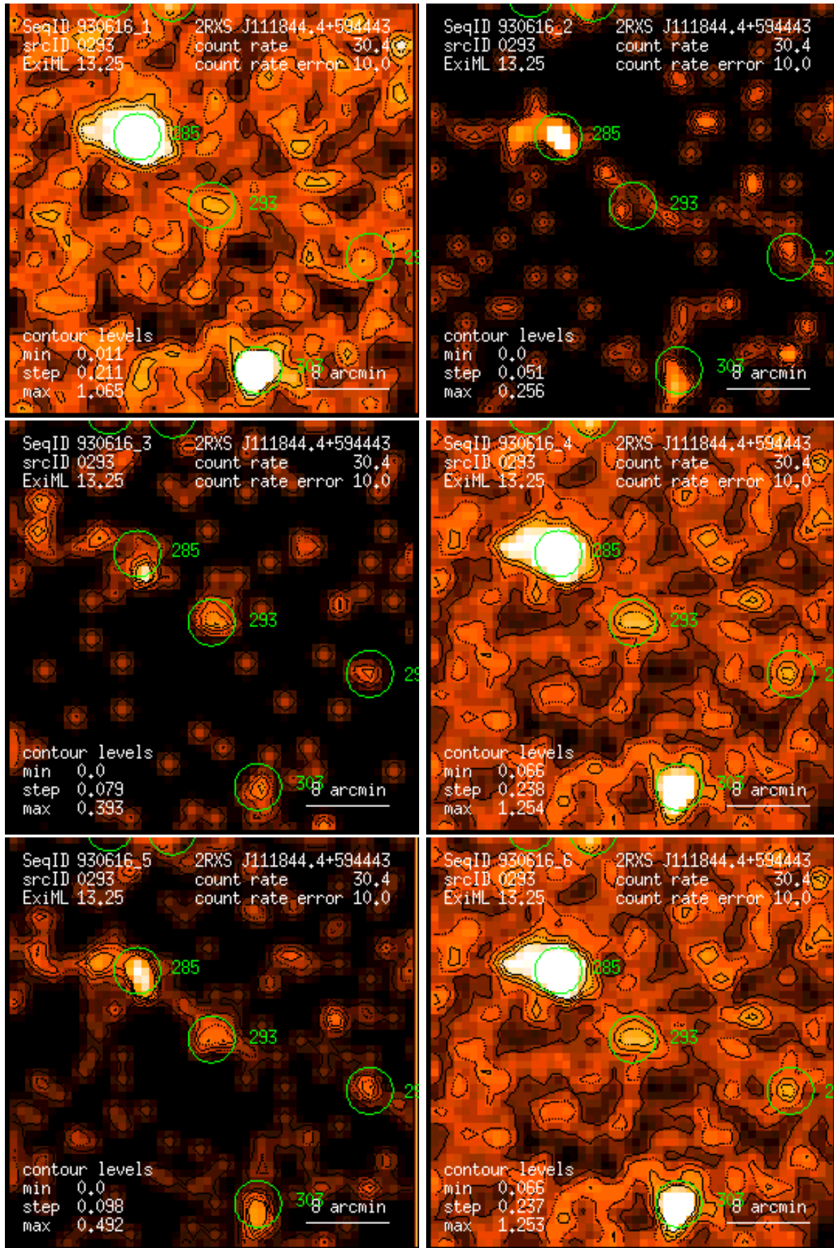
Figure 293: RASS 930616: detection 0293: band rate images, Gaussian filter: (1) PSPC channels 11 – 41, (2) 52 – 90, (3) 91 – 201, (4) 11 – 235, (5) 52 – 201, (6) 11 – 201. Broad band rates in counts/ks. Band rate contour levels in counts/ks/arcmin 2 .
