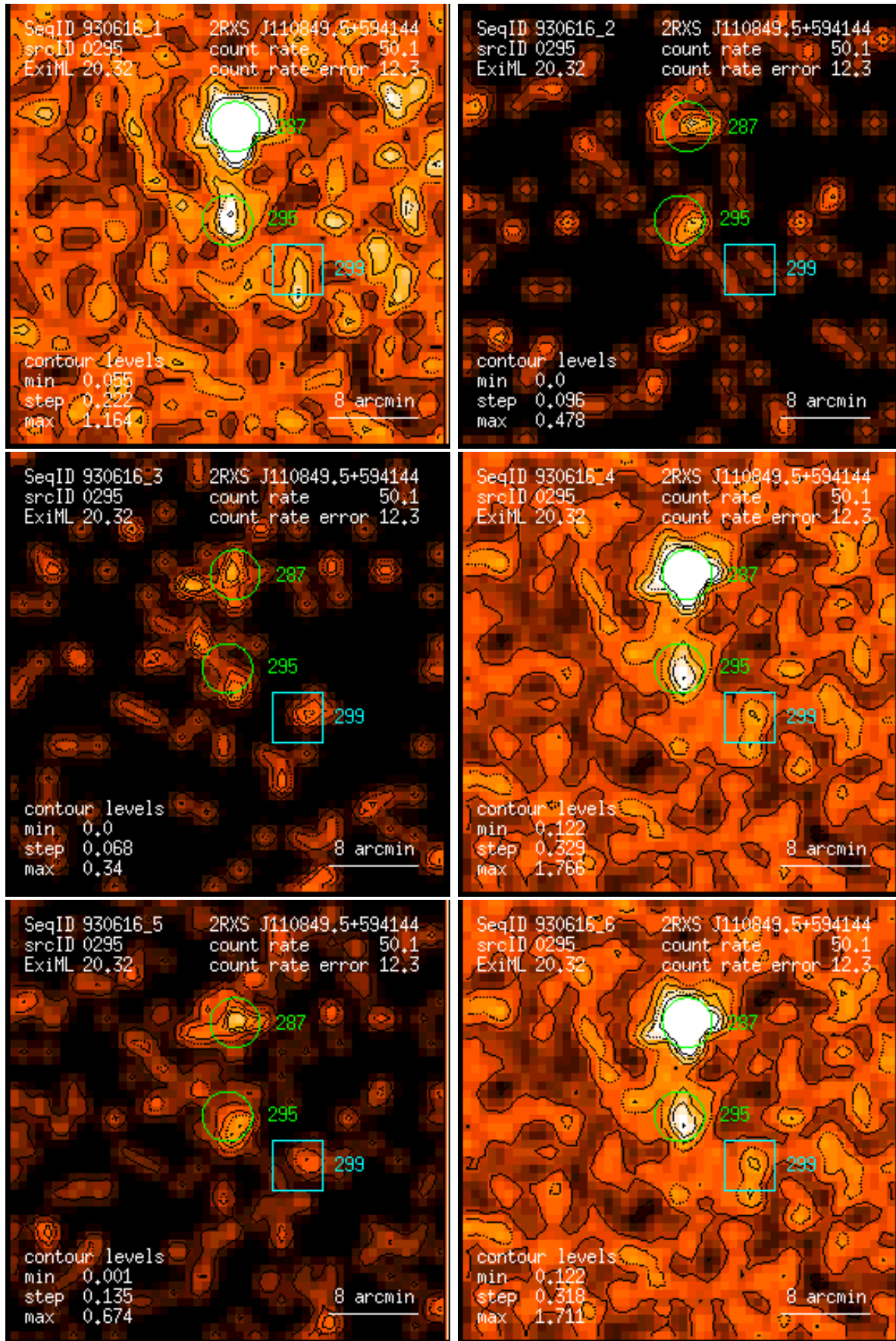
Figure 295: RASS 930616: detection 0295: band rate images, Gaussian filter: (1) PSPC channels 11 – 41, (2) 52 – 90, (3) 91 – 201, (4) 11 – 235, (5) 52 – 201, (6) 11 – 201. Broad band rates in counts/ks. Band rate contour levels in counts/ks/arcmin 2 .
