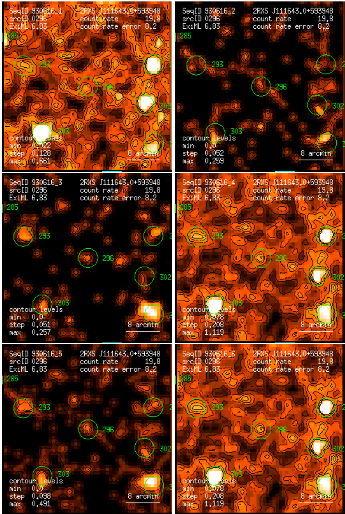
Figure 296: RASS 930616: detection 0296: band rate images, Gaussian filter: (1) PSPC channels 11 – 41, (2) 52 – 90, (3) 91 – 201, (4) 11 – 235, (5) 52 – 201, (6) 11 – 201. Broad band rates in counts/ks. Band rate contour levels in counts/ks/arcmin 2 .
