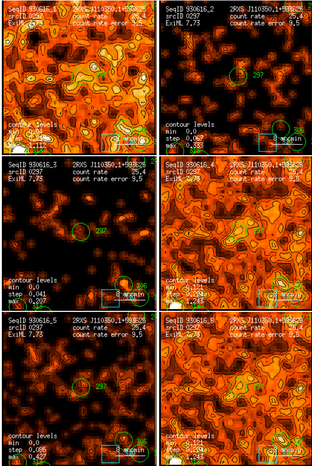
Figure 297: RASS 930616: detection 0297: band rate images, Gaussian filter: (1) PSPC channels 11 – 41, (2) 52 – 90, (3) 91 – 201, (4) 11 – 235, (5) 52 – 201, (6) 11 – 201. Broad band rates in counts/ks. Band rate contour levels in counts/ks/arcmin 2 .
