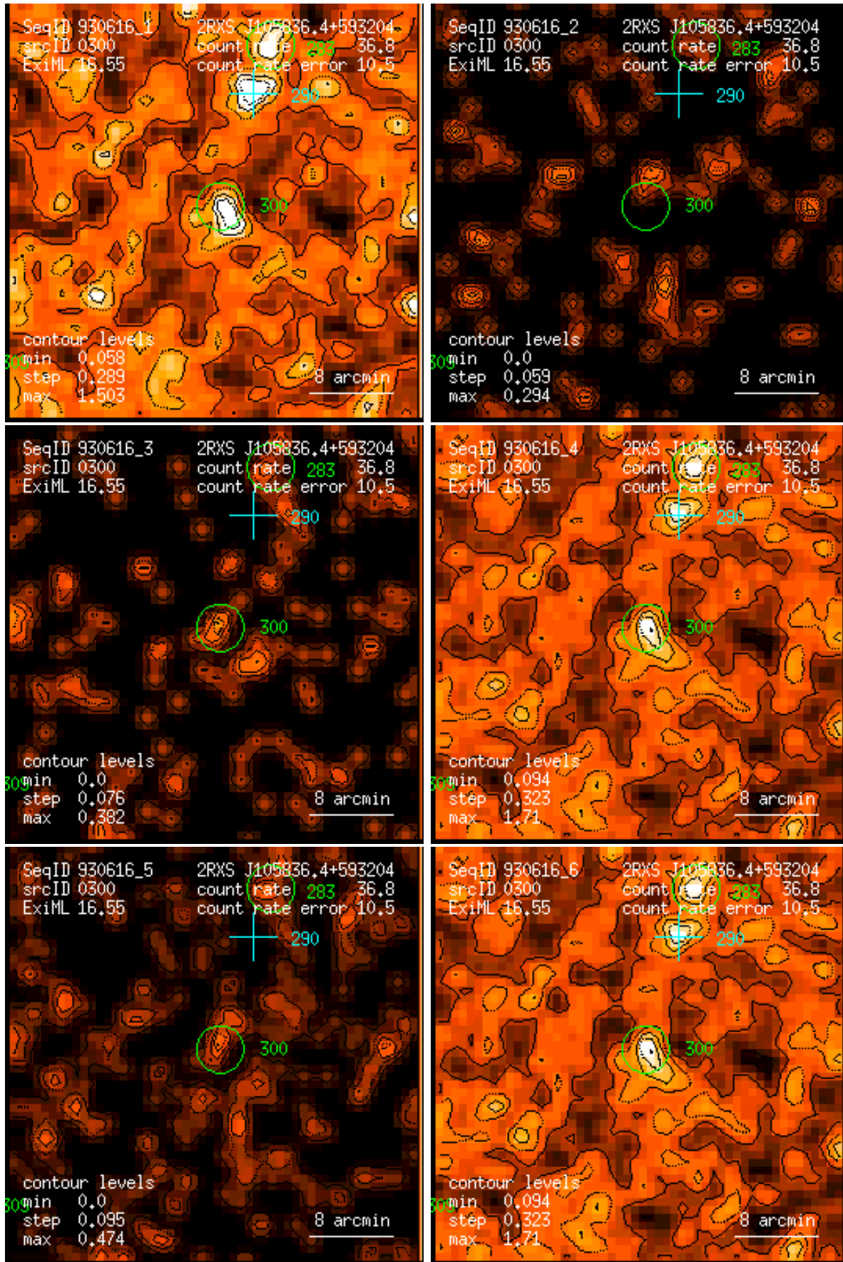
Figure 300: RASS 930616: detection 0300: band rate images, Gaussian filter: (1) PSPC channels 11 – 41, (2) 52 – 90, (3) 91 – 201, (4) 11 – 235, (5) 52 – 201, (6) 11 – 201. Broad band rates in counts/ks. Band rate contour levels in counts/ks/arcmin 2 .
