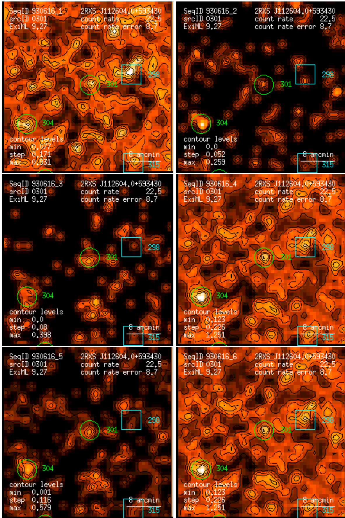
Figure 301: RASS 930616: detection 0301: band rate images, Gaussian filter: (1) PSPC channels 11 – 41, (2) 52 – 90, (3) 91 – 201, (4) 11 – 235, (5) 52 – 201, (6) 11 – 201. Broad band rates in counts/ks. Band rate contour levels in counts/ks/arcmin 2 .
