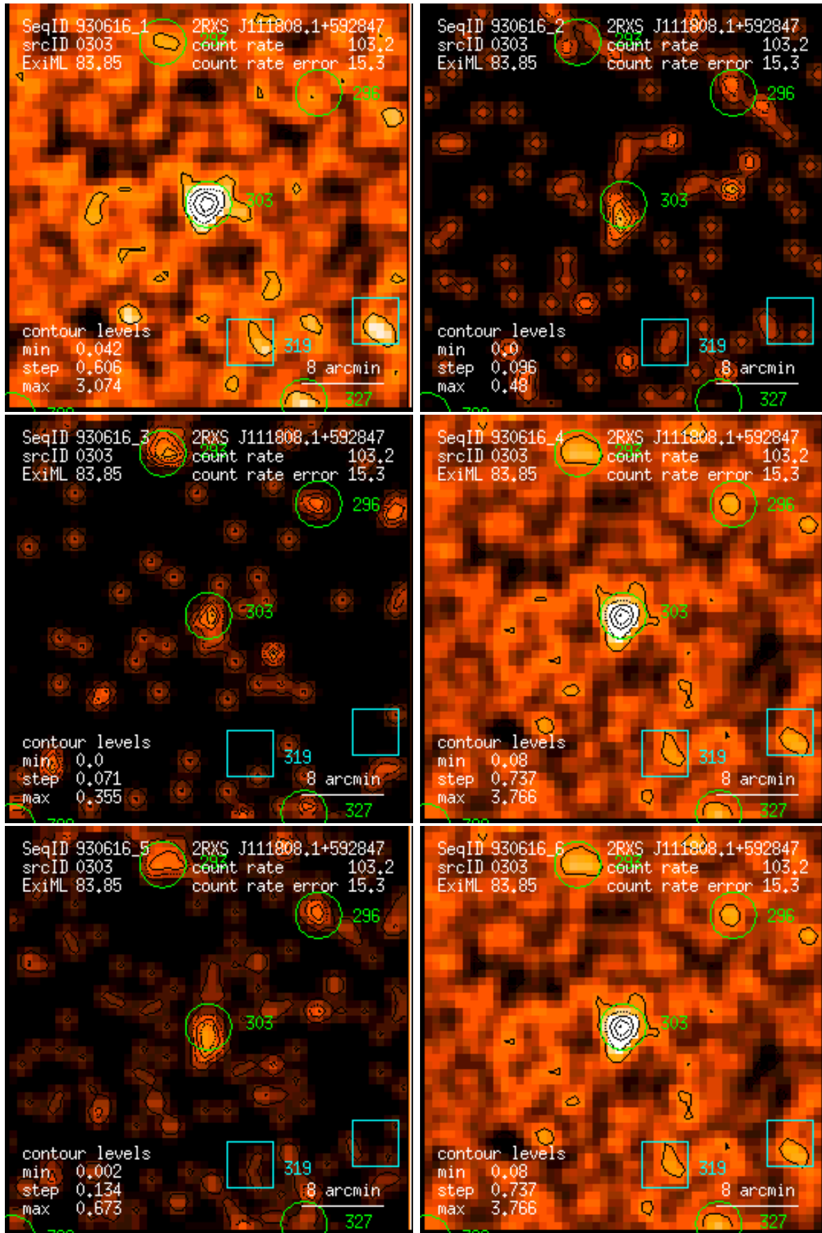
Figure 303: RASS 930616: detection 0303: band rate images, Gaussian filter: (1) PSPC channels 11 – 41, (2) 52 – 90, (3) 91 – 201, (4) 11 – 235, (5) 52 – 201, (6) 11 – 201. Broad band rates in counts/ks. Band rate contour levels in counts/ks/arcmin 2 .
