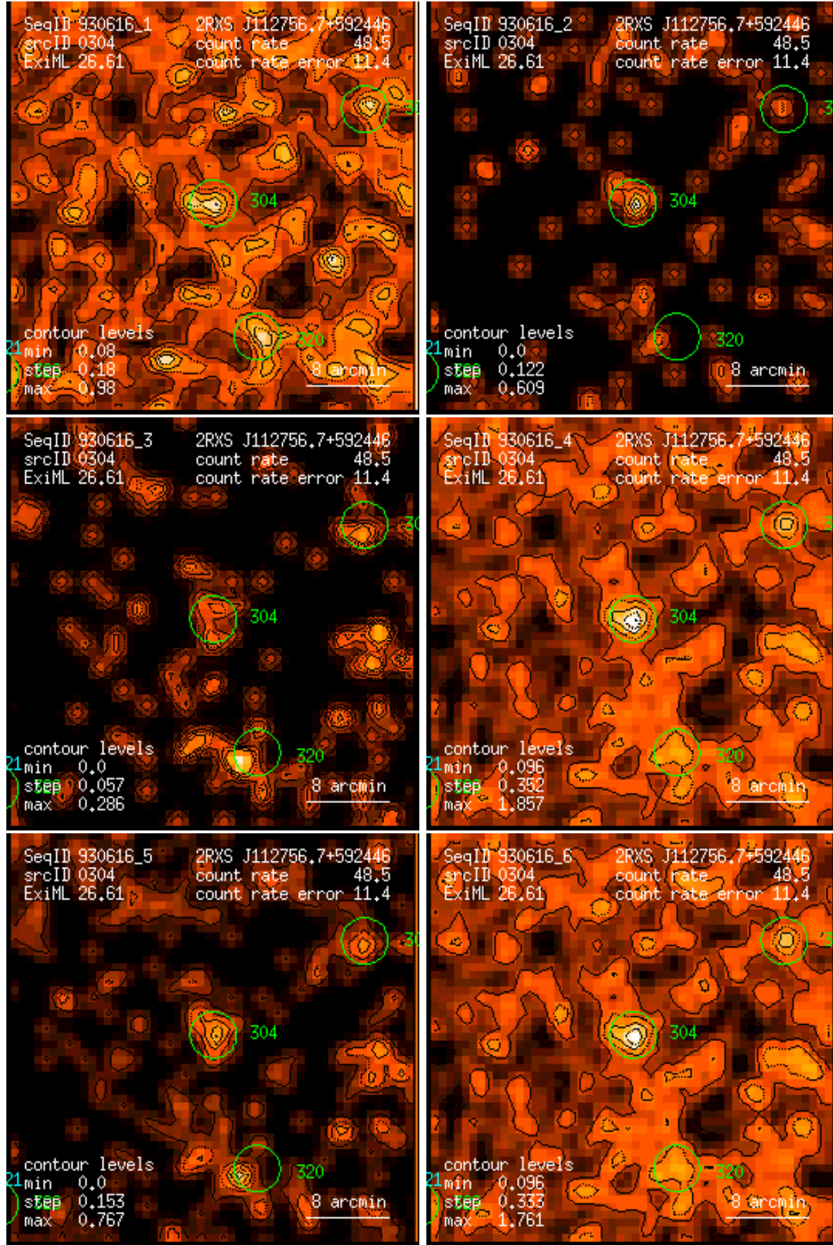
Figure 304: RASS 930616: detection 0304: band rate images, Gaussian filter: (1) PSPC channels 11 – 41, (2) 52 – 90, (3) 91 – 201, (4) 11 – 235, (5) 52 – 201, (6) 11 – 201. Broad band rates in counts/ks. Band rate contour levels in counts/ks/arcmin 2 .
