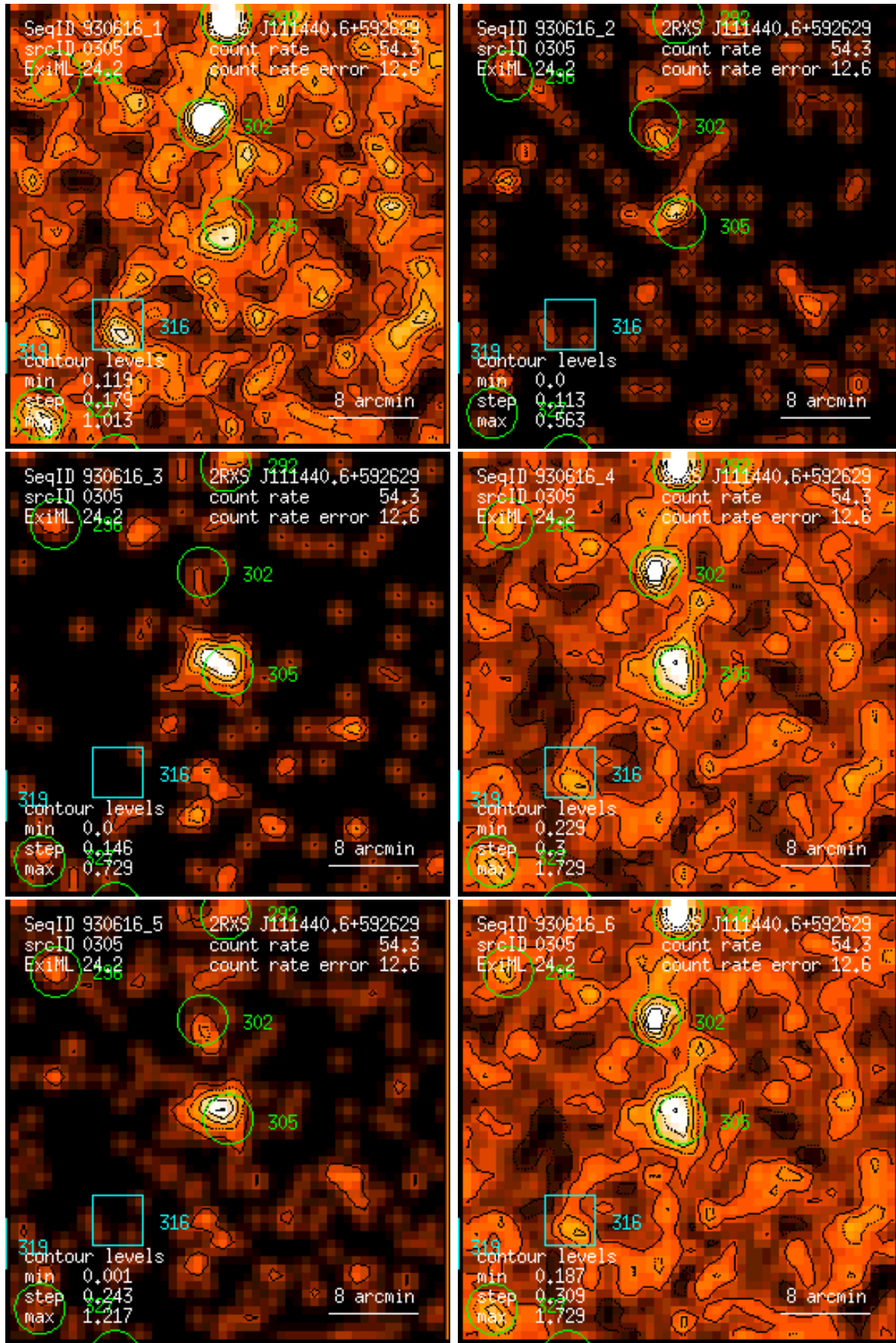
Figure 305: RASS 930616: detection 0305: band rate images, Gaussian filter: (1) PSPC channels 11 – 41, (2) 52 – 90, (3) 91 – 201, (4) 11 – 235, (5) 52 – 201, (6) 11 – 201. Broad band rates in counts/ks. Band rate contour levels in counts/ks/arcmin 2 .
