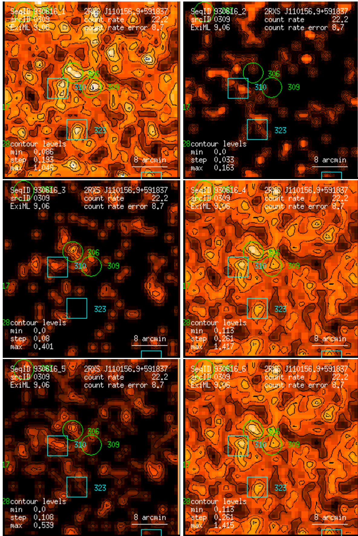
Figure 309: RASS 930616: detection 0309: band rate images, Gaussian filter: (1) PSPC channels 11 – 41, (2) 52 – 90, (3) 91 – 201, (4) 11 – 235, (5) 52 – 201, (6) 11 – 201. Broad band rates in counts/ks. Band rate contour levels in counts/ks/arcmin 2 .
