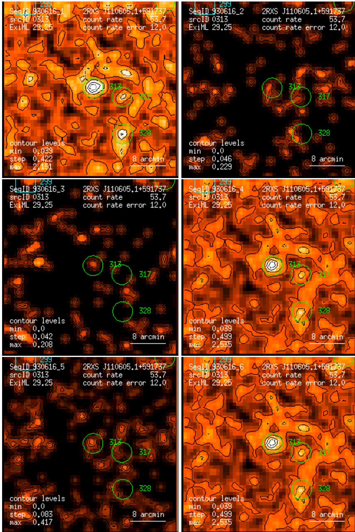
Figure 313: RASS 930616: detection 0313: band rate images, Gaussian filter: (1) PSPC channels 11 – 41, (2) 52 – 90, (3) 91 – 201, (4) 11 – 235, (5) 52 – 201, (6) 11 – 201. Broad band rates in counts/ks. Band rate contour levels in counts/ks/arcmin 2 .
