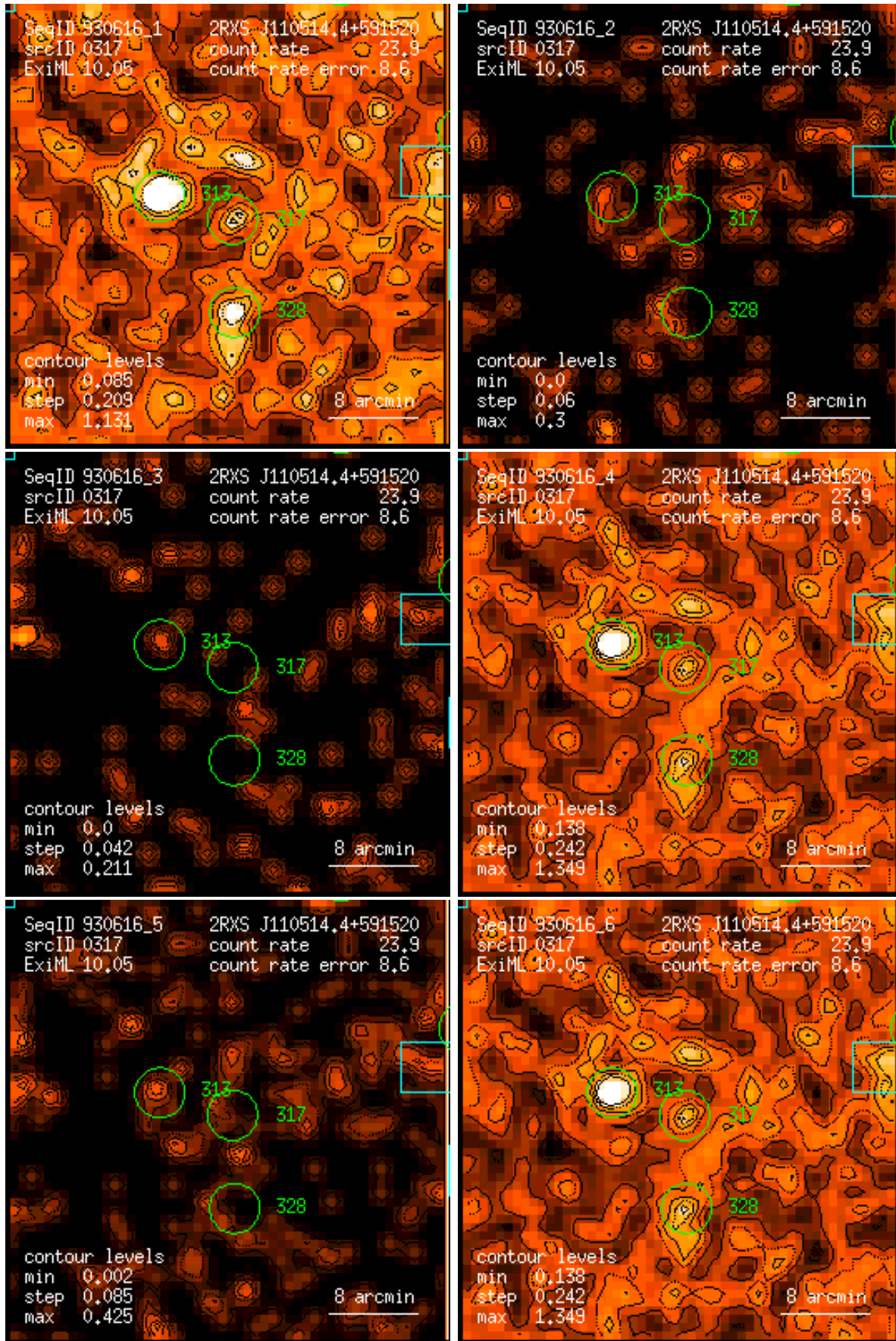
Figure 317: RASS 930616: detection 0317: band rate images, Gaussian filter: (1) PSPC channels 11 – 41, (2) 52 – 90, (3) 91 – 201, (4) 11 – 235, (5) 52 – 201, (6) 11 – 201. Broad band rates in counts/ks. Band rate contour levels in counts/ks/arcmin 2 .
