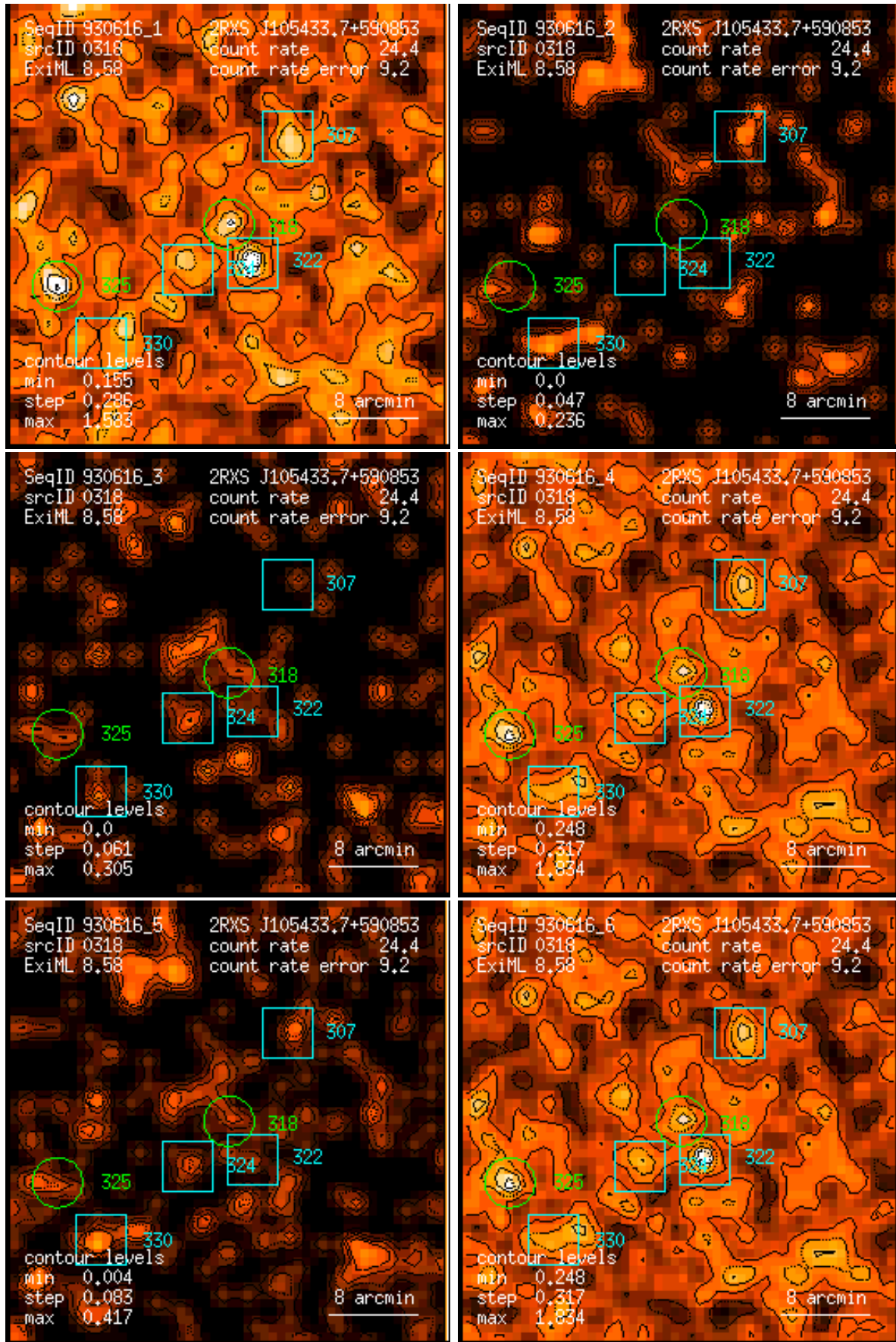
Figure 318: RASS 930616: detection 0318: band rate images, Gaussian filter: (1) PSPC channels 11 – 41, (2) 52 – 90, (3) 91 – 201, (4) 11 – 235, (5) 52 – 201, (6) 11 – 201. Broad band rates in counts/ks. Band rate contour levels in counts/ks/arcmin 2 .
