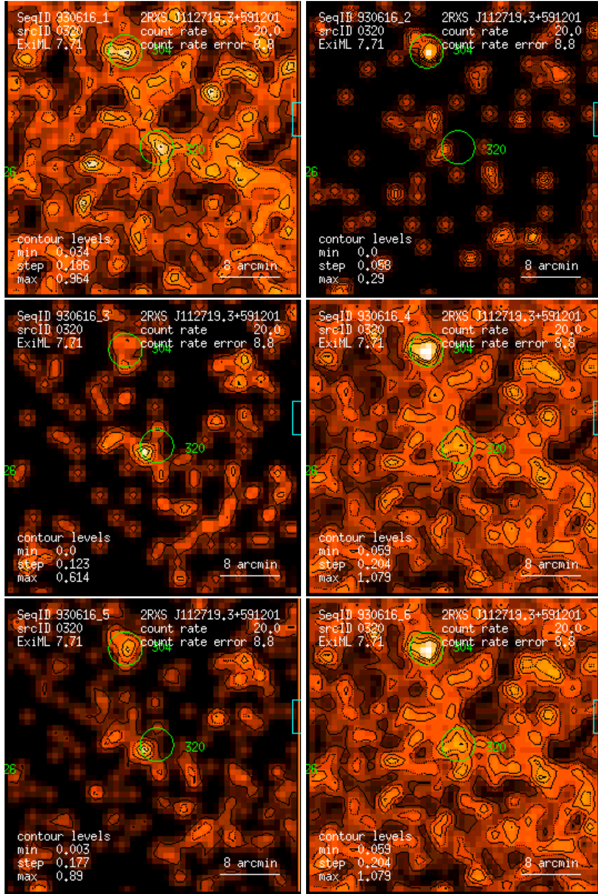
Figure 320: RASS 930616: detection 0320: band rate images, Gaussian filter: (1) PSPC channels 11 – 41, (2) 52 – 90, (3) 91 – 201, (4) 11 – 235, (5) 52 – 201, (6) 11 – 201. Broad band rates in counts/ks. Band rate contour levels in counts/ks/arcmin 2 .
