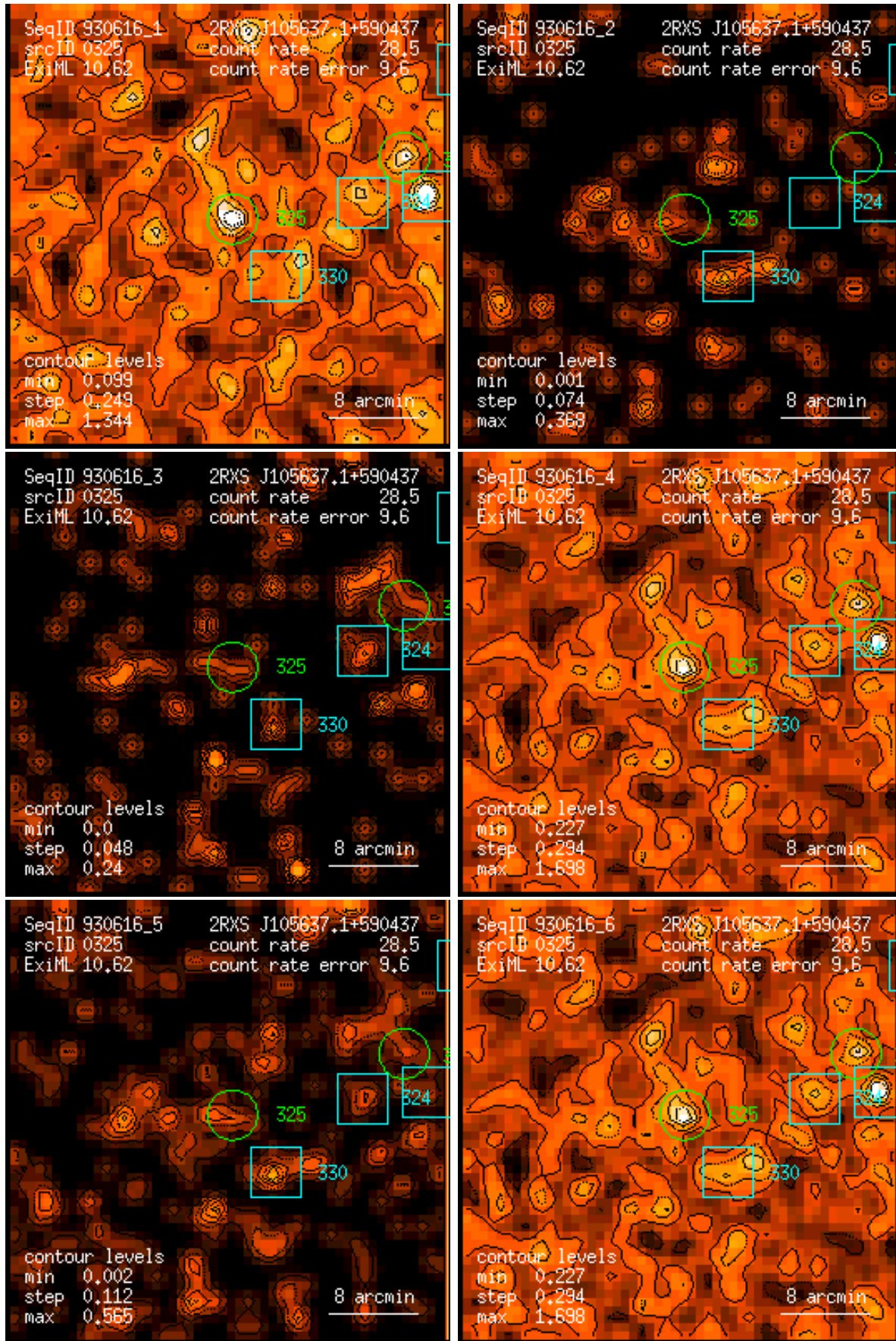
Figure 325: RASS 930616: detection 0325: band rate images, Gaussian filter: (1) PSPC channels 11 – 41, (2) 52 – 90, (3) 91 – 201, (4) 11 – 235, (5) 52 – 201, (6) 11 – 201. Broad band rates in counts/ks. Band rate contour levels in counts/ks/arcmin 2 .
