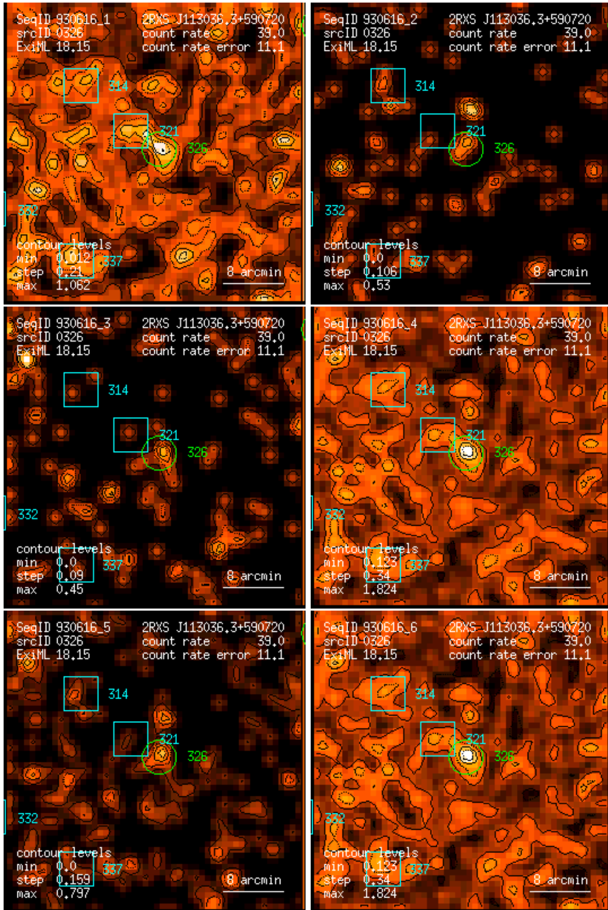
Figure 326: RASS 930616: detection 0326: band rate images, Gaussian filter: (1) PSPC channels 11 – 41, (2) 52 – 90, (3) 91 – 201, (4) 11 – 235, (5) 52 – 201, (6) 11 – 201. Broad band rates in counts/ks. Band rate contour levels in counts/ks/arcmin 2 .
