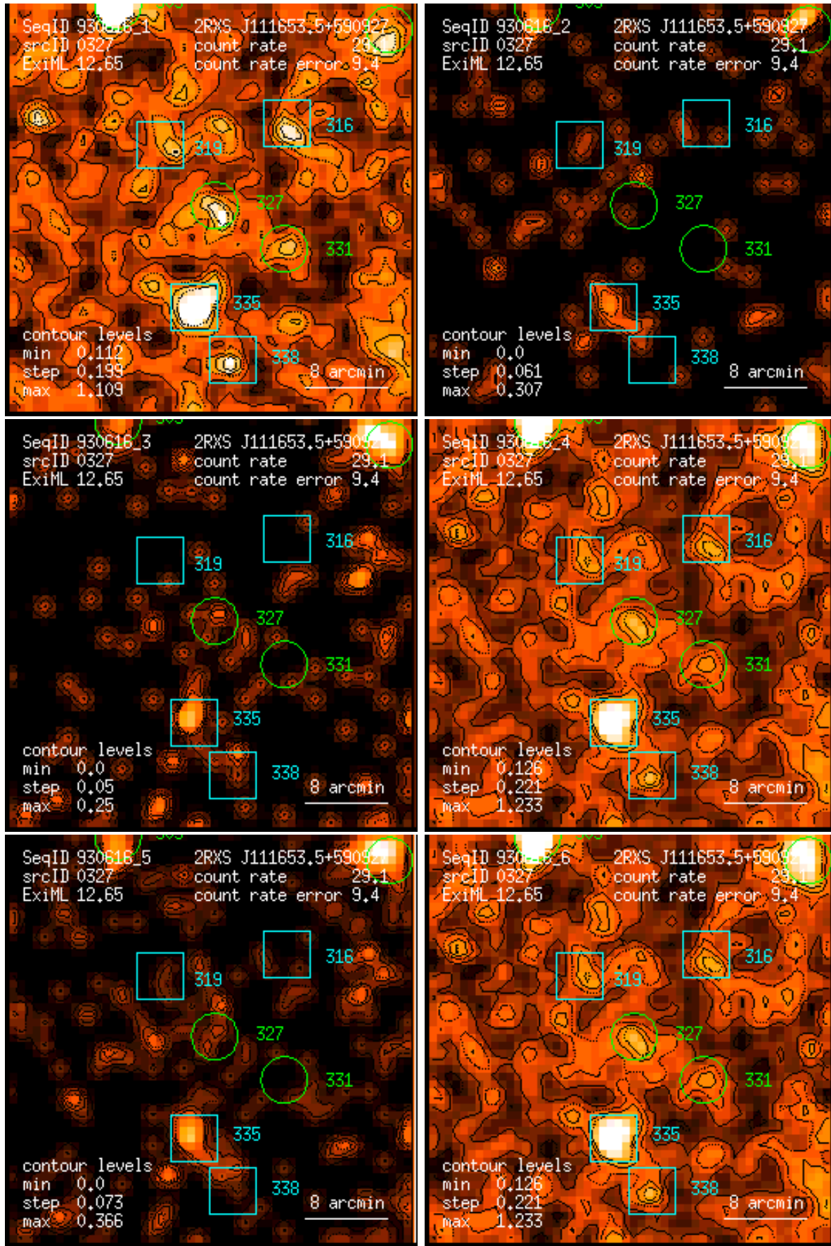
Figure 327: RASS 930616: detection 0327: band rate images, Gaussian filter: (1) PSPC channels 11 – 41, (2) 52 – 90, (3) 91 – 201, (4) 11 – 235, (5) 52 – 201, (6) 11 – 201. Broad band rates in counts/ks. Band rate contour levels in counts/ks/arcmin 2 .
