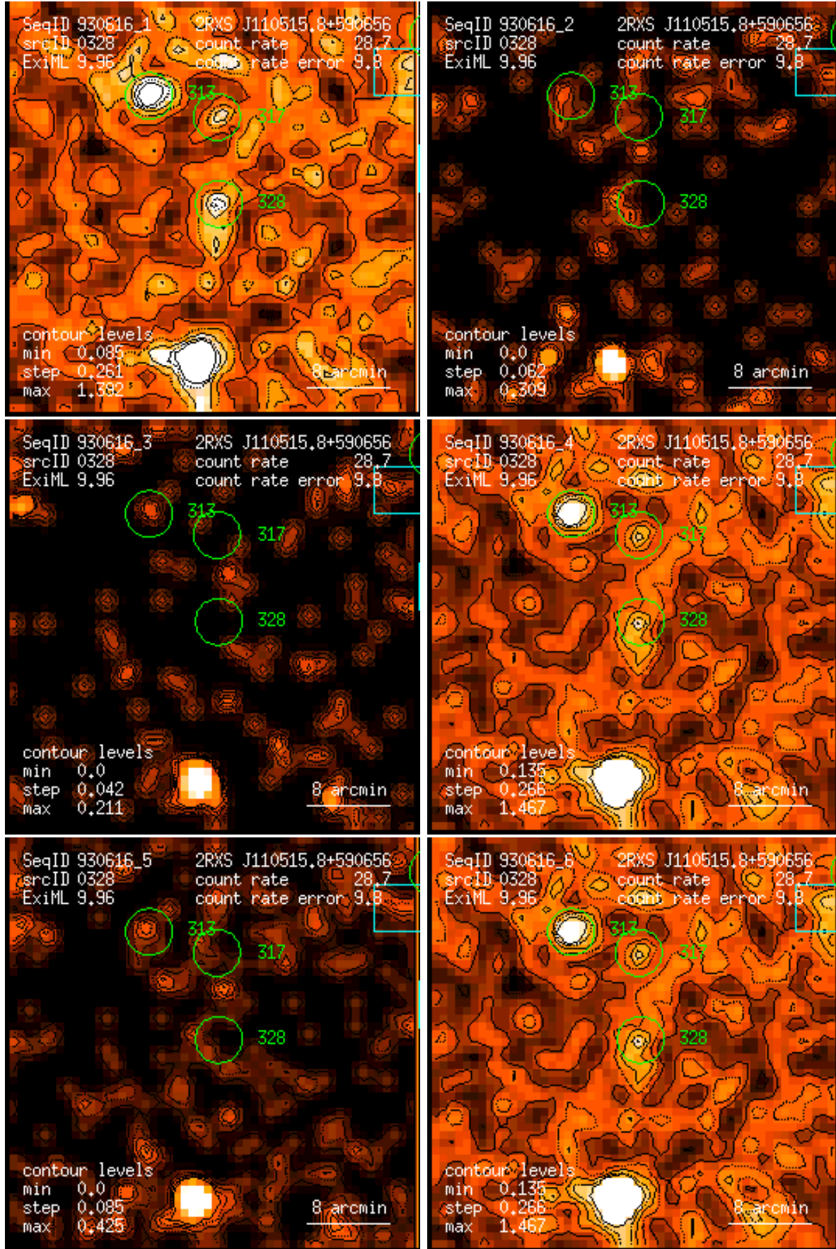
Figure 328: RASS 930616: detection 0328: band rate images, Gaussian filter: (1) PSPC channels 11 – 41, (2) 52 – 90, (3) 91 – 201, (4) 11 – 235, (5) 52 – 201, (6) 11 – 201. Broad band rates in counts/ks. Band rate contour levels in counts/ks/arcmin 2 .
