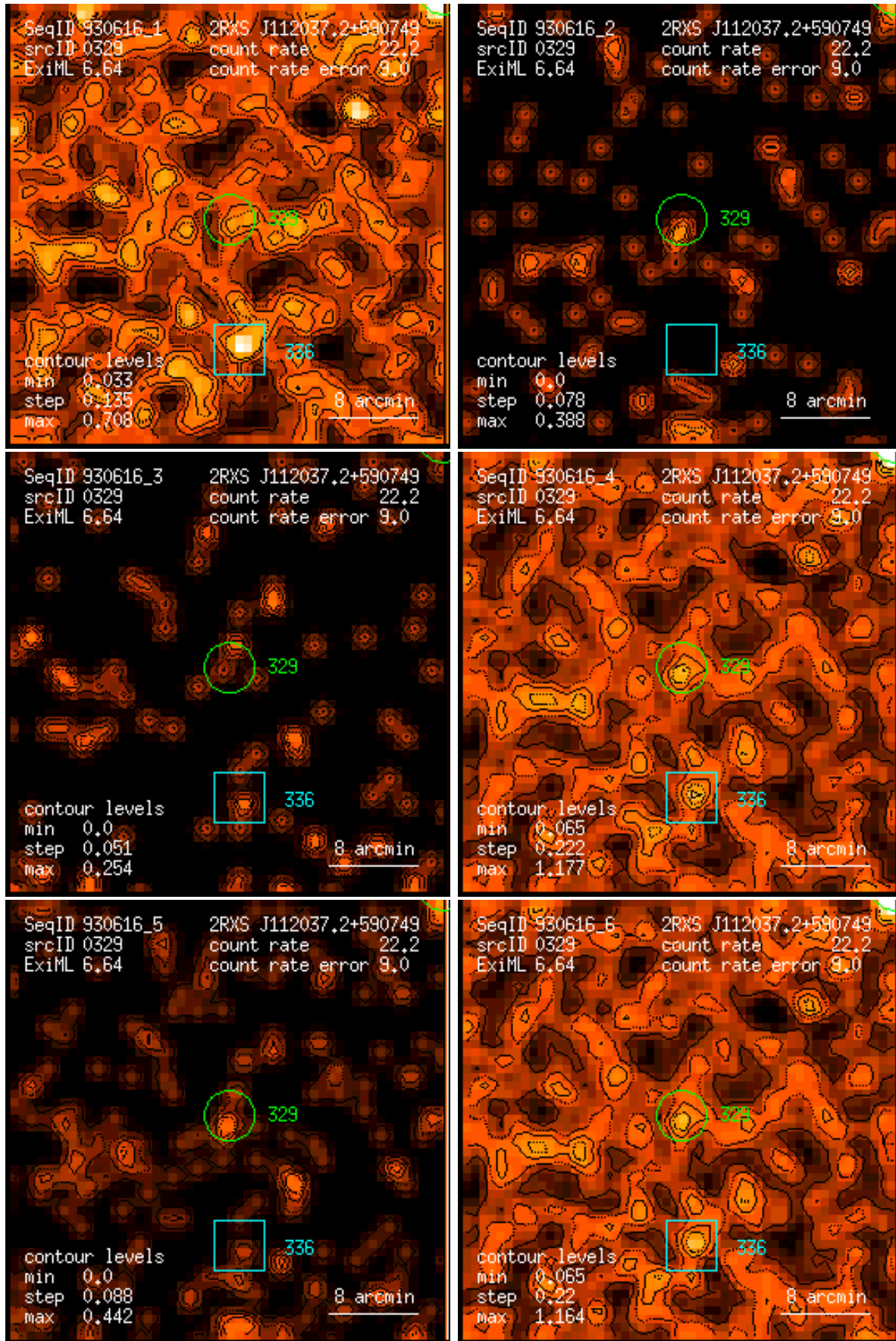
Figure 329: RASS 930616: detection 0329: band rate images, Gaussian filter: (1) PSPC channels 11 – 41, (2) 52 – 90, (3) 91 – 201, (4) 11 – 235, (5) 52 – 201, (6) 11 – 201. Broad band rates in counts/ks. Band rate contour levels in counts/ks/arcmin 2 .
