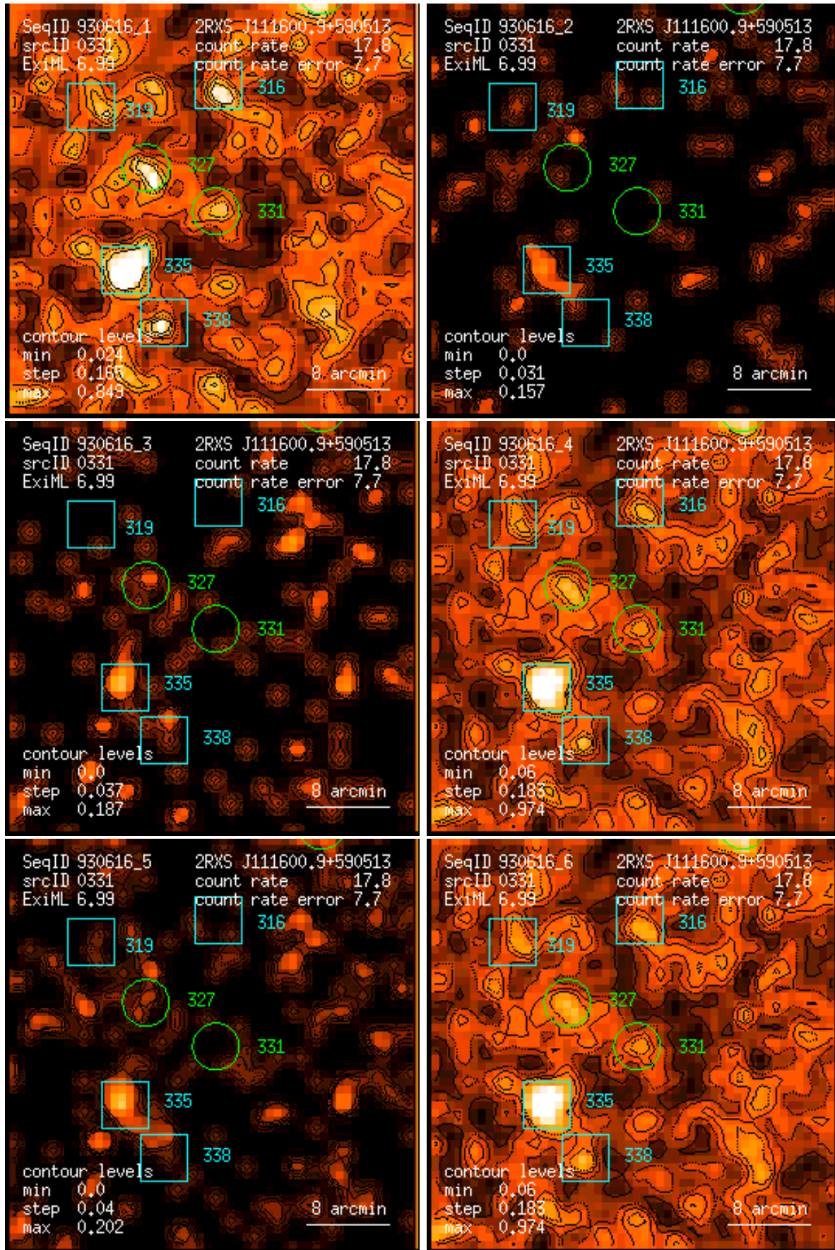
Figure 331: RASS 930616: detection 0331: band rate images, Gaussian filter: (1) PSPC channels 11 – 41, (2) 52 – 90, (3) 91 – 201, (4) 11 – 235, (5) 52 – 201, (6) 11 – 201. Broad band rates in counts/ks. Band rate contour levels in counts/ks/arcmin 2 .
