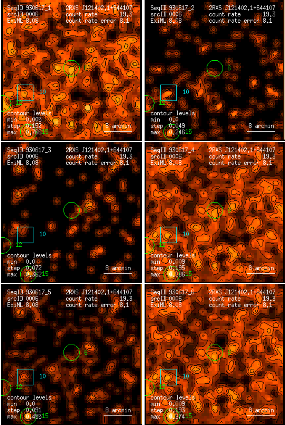
Figure 6: RASS 930617: detection 0006: band rate images, Gaussian filter: (1) PSPC channels 11 – 41, (2) 52 – 90, (3) 91 – 201, (4) 11 – 235, (5) 52 – 201, (6) 11 – 201. Broad band rates in counts/ks. Band rate contour levels in counts/ks/arcmin 2 .
