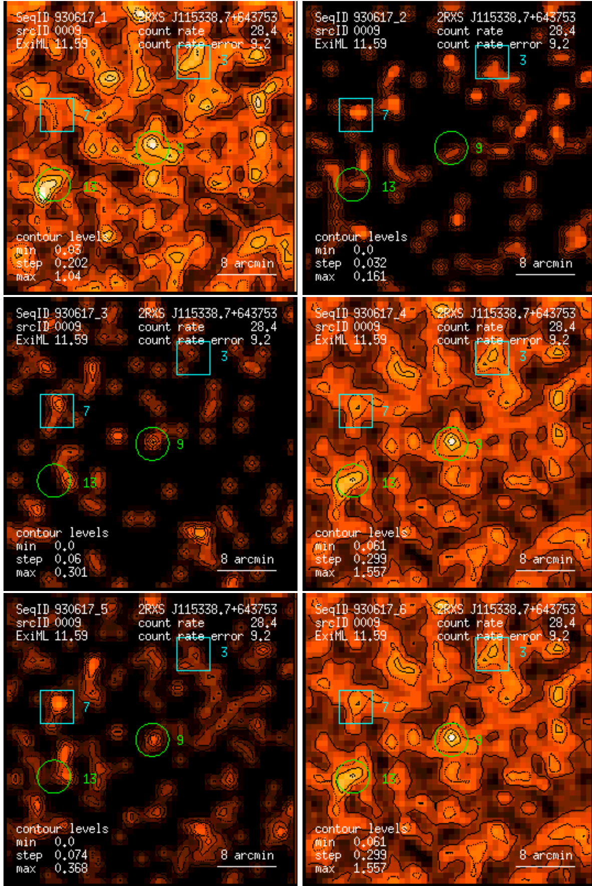
Figure 9: RASS 930617: detection 0009: band rate images, Gaussian filter: (1) PSPC channels 11 – 41, (2) 52 – 90, (3) 91 – 201, (4) 11 – 235, (5) 52 – 201, (6) 11 – 201. Broad band rates in counts/ks. Band rate contour levels in counts/ks/arcmin 2 .
