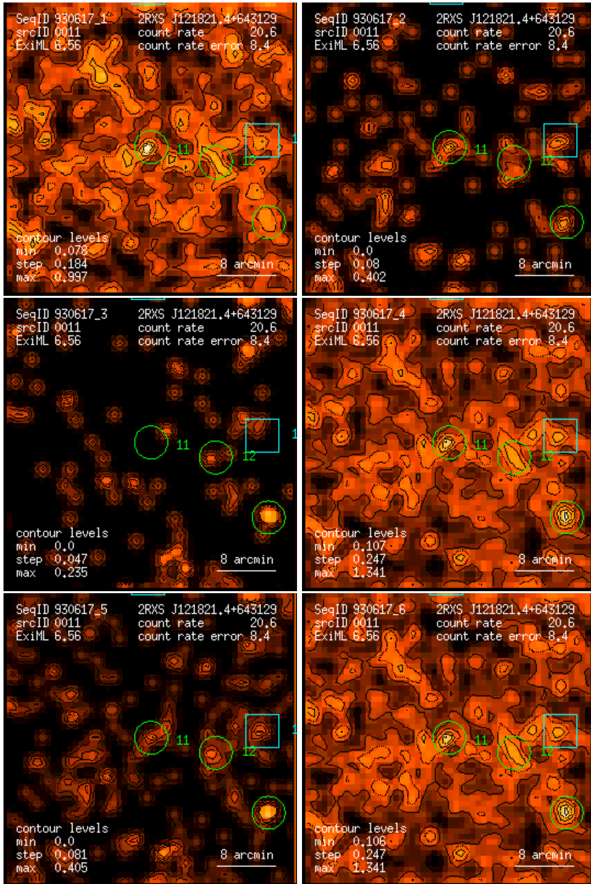
Figure 11: RASS 930617: detection 0011: band rate images, Gaussian filter: (1) PSPC channels 11 – 41, (2) 52 – 90, (3) 91 – 201, (4) 11 – 235, (5) 52 – 201, (6) 11 – 201. Broad band rates in counts/ks. Band rate contour levels in counts/ks/arcmin 2 .
