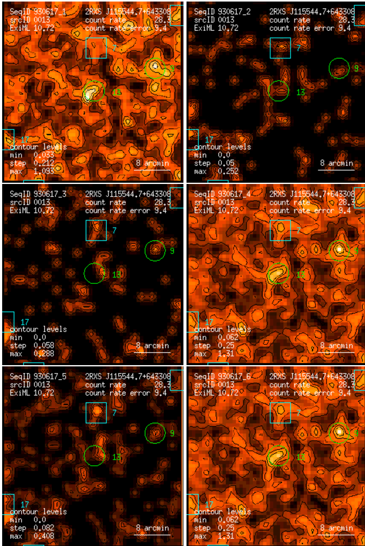
Figure 13: RASS 930617: detection 0013: band rate images, Gaussian filter: (1) PSPC channels 11 – 41, (2) 52 – 90, (3) 91 – 201, (4) 11 – 235, (5) 52 – 201, (6) 11 – 201. Broad band rates in counts/ks. Band rate contour levels in counts/ks/arcmin 2 .
