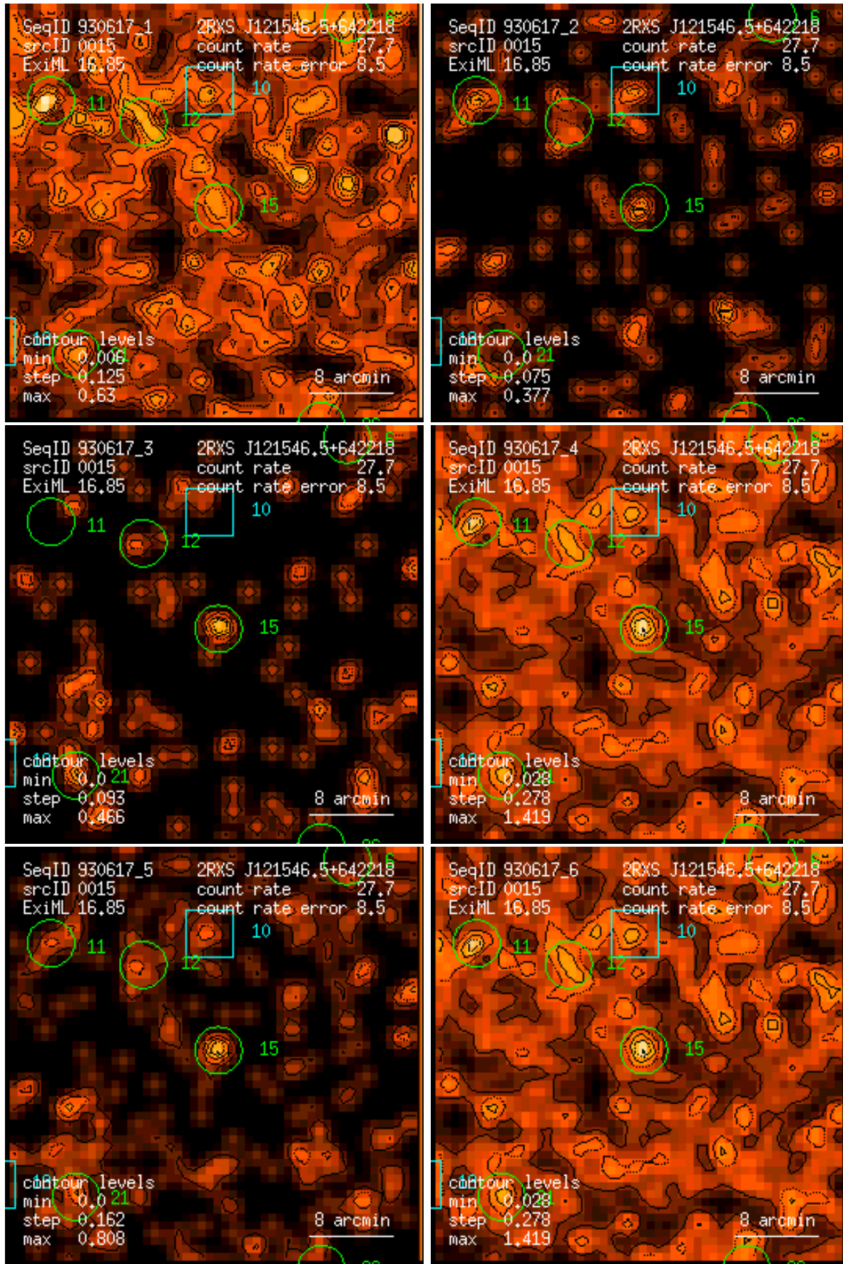
Figure 15: RASS 930617: detection 0015: band rate images, Gaussian filter: (1) PSPC channels 11 – 41, (2) 52 – 90, (3) 91 – 201, (4) 11 – 235, (5) 52 – 201, (6) 11 – 201. Broad band rates in counts/ks. Band rate contour levels in counts/ks/arcmin 2 .
