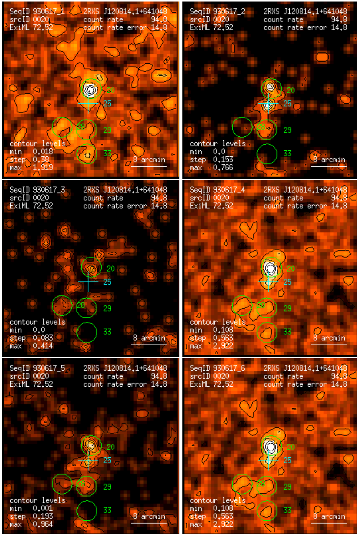
Figure 20: RASS 930617: detection 0020: band rate images, Gaussian filter: (1) PSPC channels 11 – 41, (2) 52 – 90, (3) 91 – 201, (4) 11 – 235, (5) 52 – 201, (6) 11 – 201. Broad band rates in counts/ks. Band rate contour levels in counts/ks/arcmin 2 .
