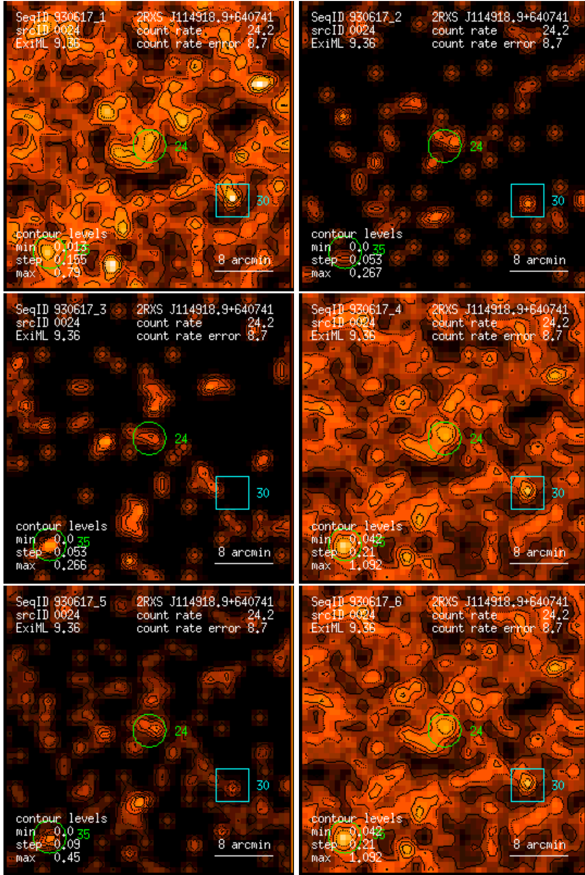
Figure 24: RASS 930617: detection 0024: band rate images, Gaussian filter: (1) PSPC channels 11 – 41, (2) 52 – 90, (3) 91 – 201, (4) 11 – 235, (5) 52 – 201, (6) 11 – 201. Broad band rates in counts/ks. Band rate contour levels in counts/ks/arcmin 2 .
