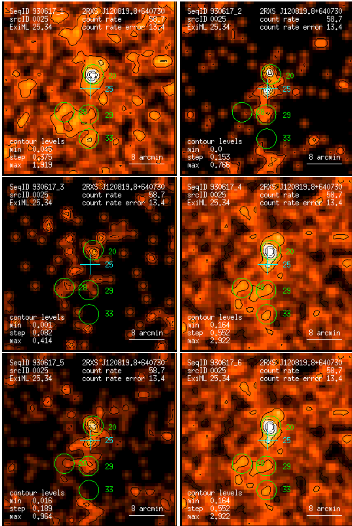
Figure 25: RASS 930617: detection 0025: band rate images, Gaussian filter: (1) PSPC channels 11 – 41, (2) 52 – 90, (3) 91 – 201, (4) 11 – 235, (5) 52 – 201, (6) 11 – 201. Broad band rates in counts/ks. Band rate contour levels in counts/ks/arcmin 2 .
