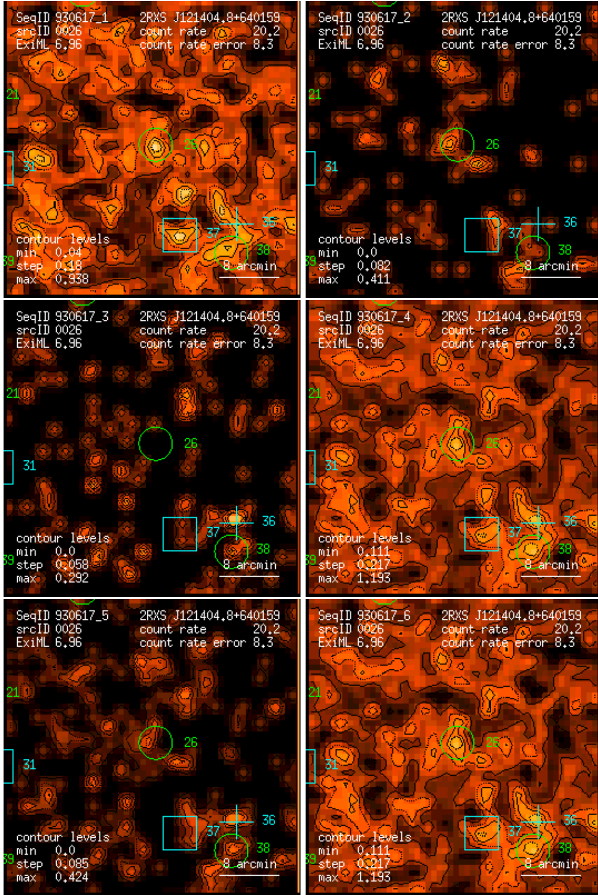
Figure 26: RASS 930617: detection 0026: band rate images, Gaussian filter: (1) PSPC channels 11 – 41, (2) 52 – 90, (3) 91 – 201, (4) 11 – 235, (5) 52 – 201, (6) 11 – 201. Broad band rates in counts/ks. Band rate contour levels in counts/ks/arcmin 2 .
