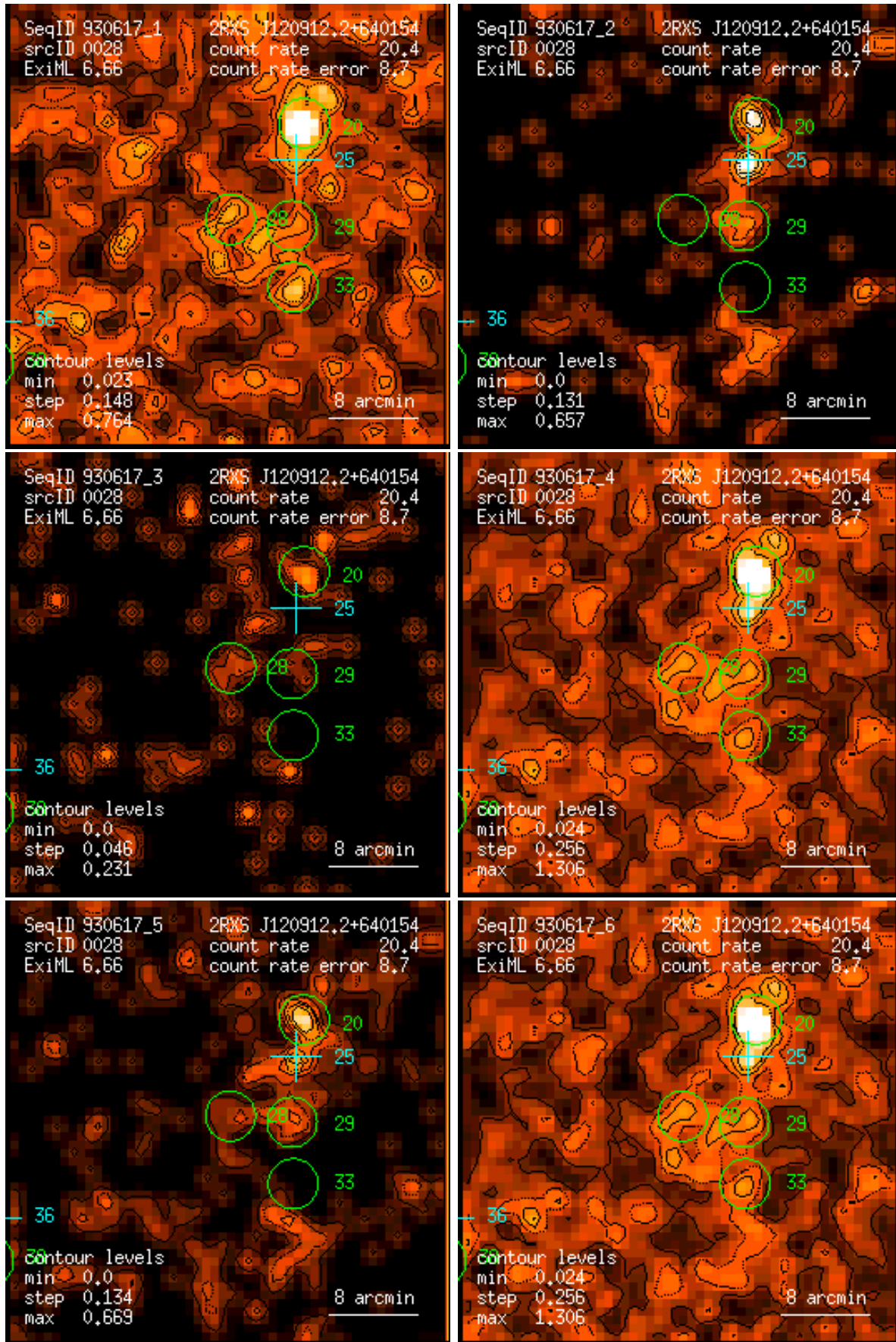
Figure 28: RASS 930617: detection 0028: band rate images, Gaussian filter: (1) PSPC channels 11 – 41, (2) 52 – 90, (3) 91 – 201, (4) 11 – 235, (5) 52 – 201, (6) 11 – 201. Broad band rates in counts/ks. Band rate contour levels in counts/ks/arcmin 2 .
