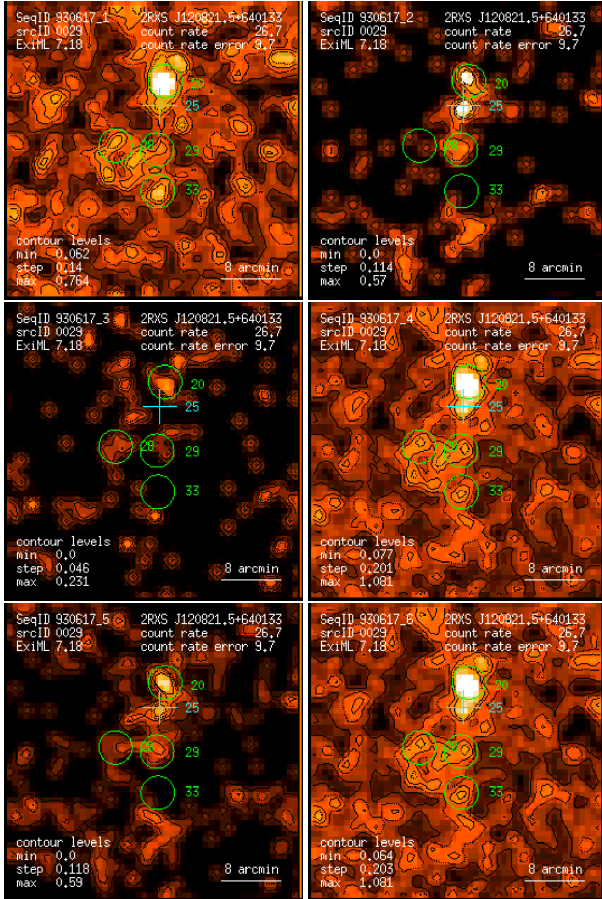
Figure 29: RASS 930617: detection 0029: band rate images, Gaussian filter: (1) PSPC channels 11 – 41, (2) 52 – 90, (3) 91 – 201, (4) 11 – 235, (5) 52 – 201, (6) 11 – 201. Broad band rates in counts/ks. Band rate contour levels in counts/ks/arcmin 2 .
