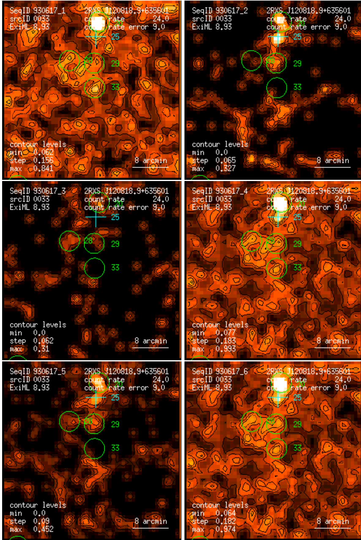
Figure 33: RASS 930617: detection 0033: band rate images, Gaussian filter: (1) PSPC channels 11 – 41, (2) 52 – 90, (3) 91 – 201, (4) 11 – 235, (5) 52 – 201, (6) 11 – 201. Broad band rates in counts/ks. Band rate contour levels in counts/ks/arcmin 2 .
