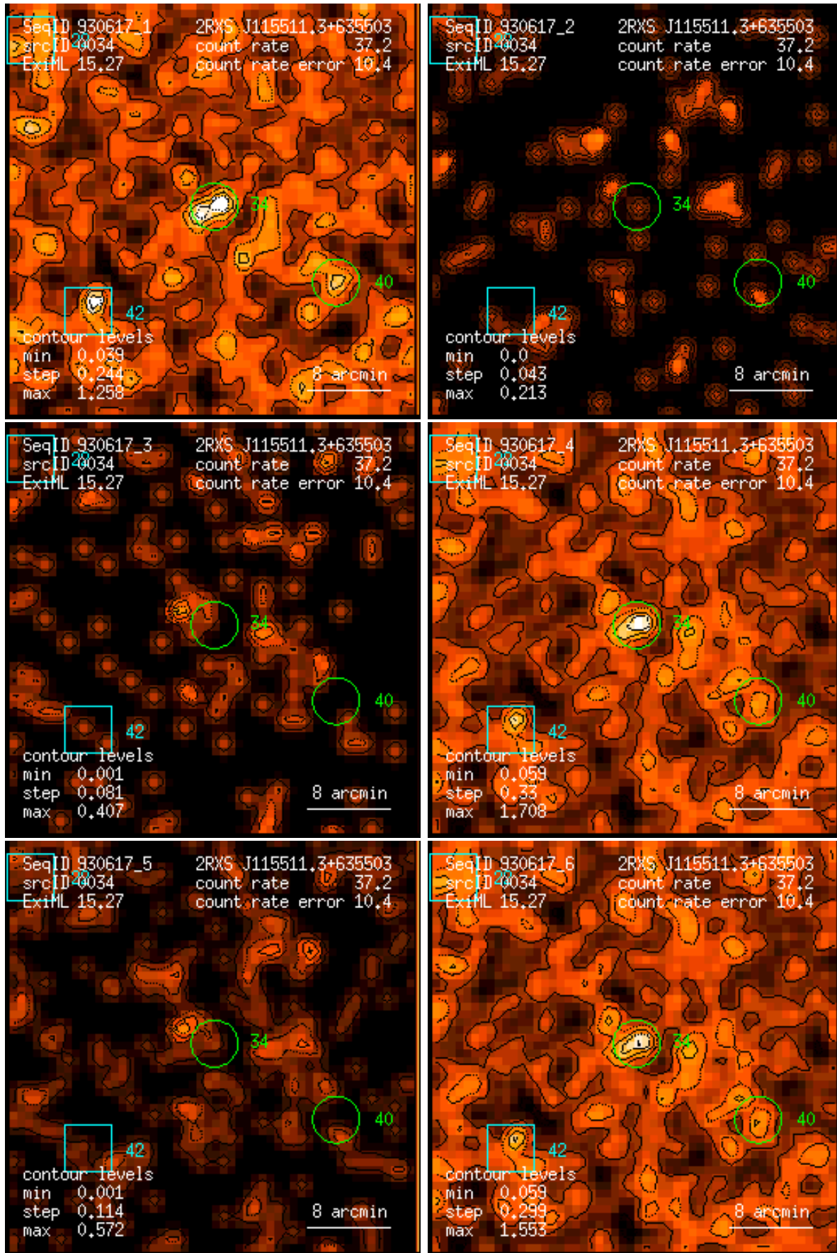
Figure 34: RASS 930617: detection 0034: band rate images, Gaussian filter: (1) PSPC channels 11 – 41, (2) 52 – 90, (3) 91 – 201, (4) 11 – 235, (5) 52 – 201, (6) 11 – 201. Broad band rates in counts/ks. Band rate contour levels in counts/ks/arcmin 2 .
