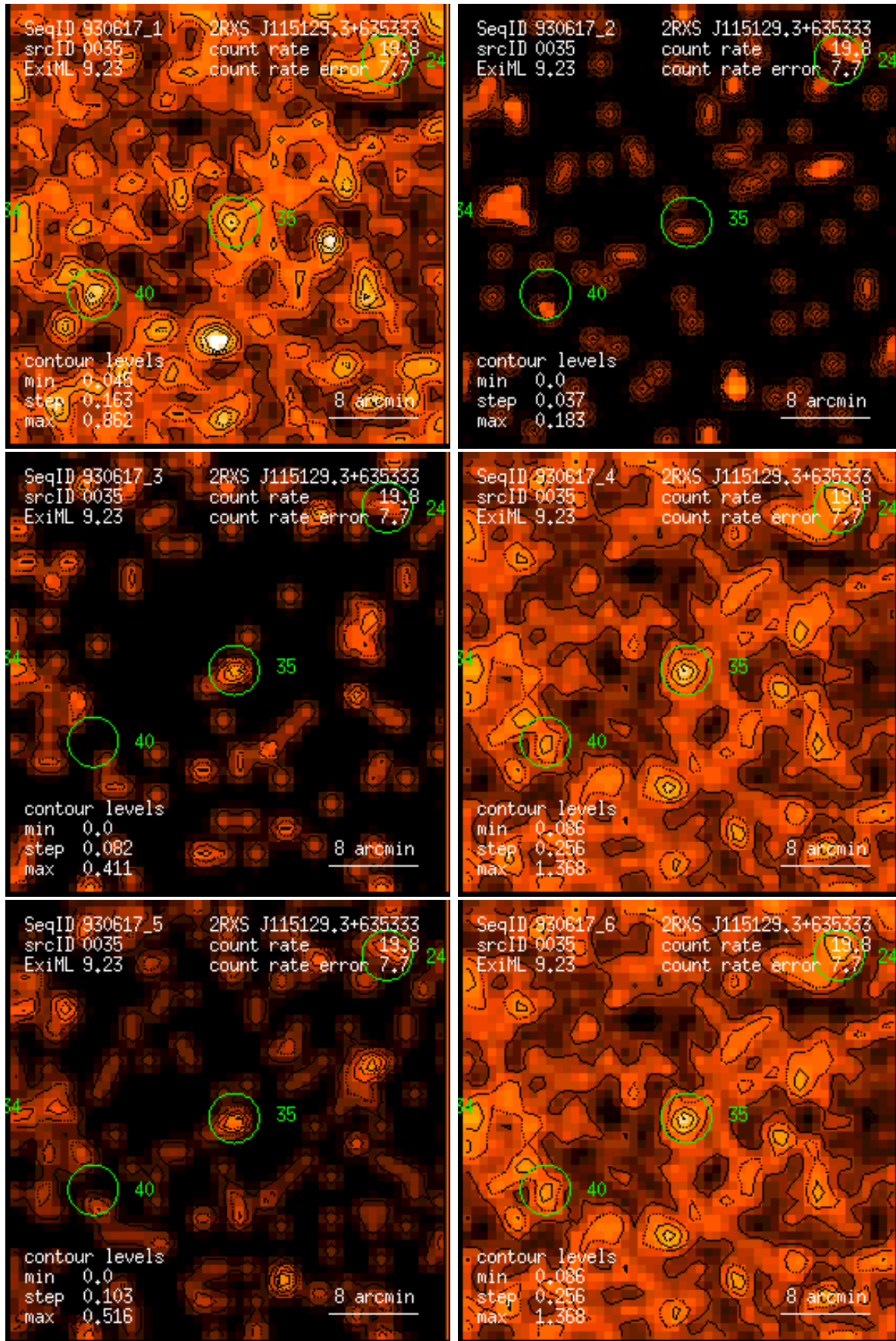
Figure 35: RASS 930617: detection 0035: band rate images, Gaussian filter: (1) PSPC channels 11 – 41, (2) 52 – 90, (3) 91 – 201, (4) 11 – 235, (5) 52 – 201, (6) 11 – 201. Broad band rates in counts/ks. Band rate contour levels in counts/ks/arcmin 2 .
