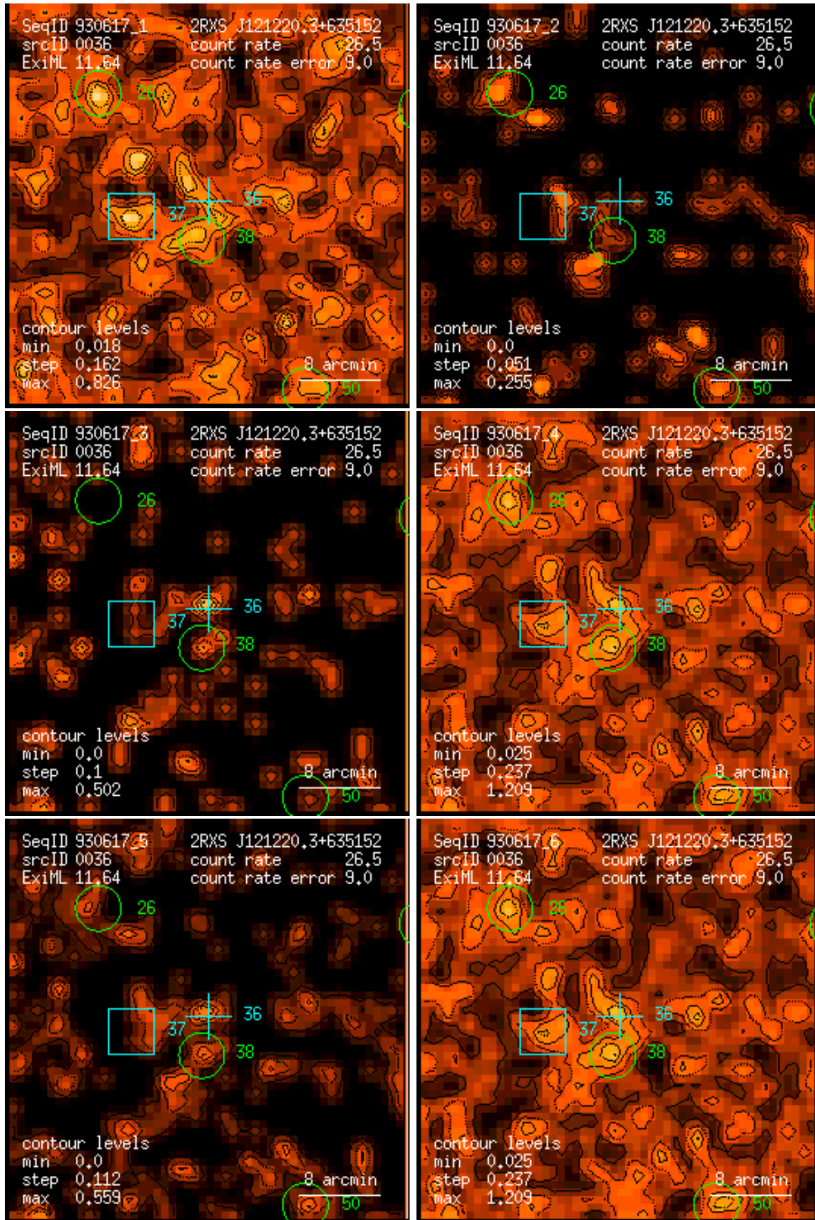
Figure 36: RASS 930617: detection 0036: band rate images, Gaussian filter: (1) PSPC channels 11 – 41, (2) 52 – 90, (3) 91 – 201, (4) 11 – 235, (5) 52 – 201, (6) 11 – 201. Broad band rates in counts/ks. Band rate contour levels in counts/ks/arcmin 2 .
