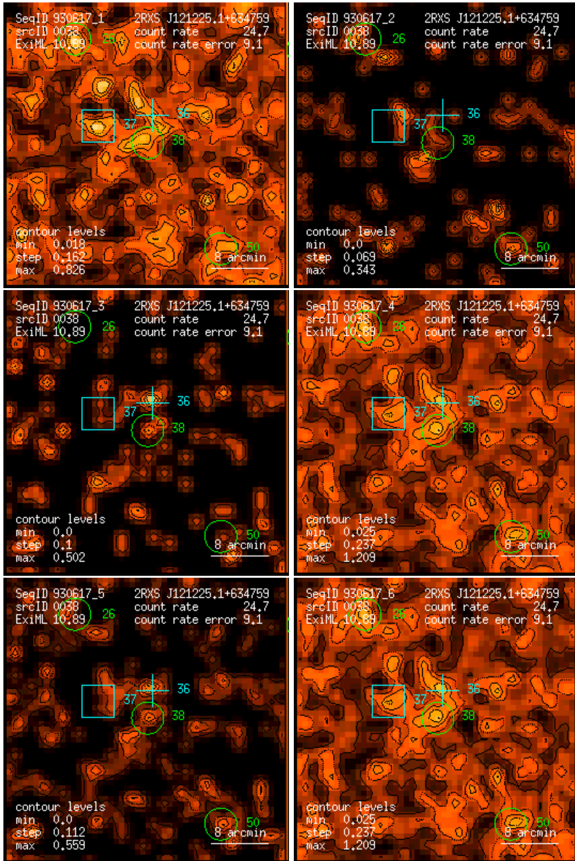
Figure 38: RASS 930617: detection 0038: band rate images, Gaussian filter: (1) PSPC channels 11 – 41, (2) 52 – 90, (3) 91 – 201, (4) 11 – 235, (5) 52 – 201, (6) 11 – 201. Broad band rates in counts/ks. Band rate contour levels in counts/ks/arcmin 2 .
